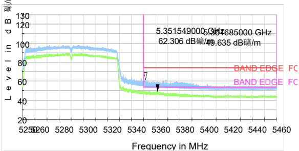
802.11ac VHT80 -Channel 58: Peak + Average
