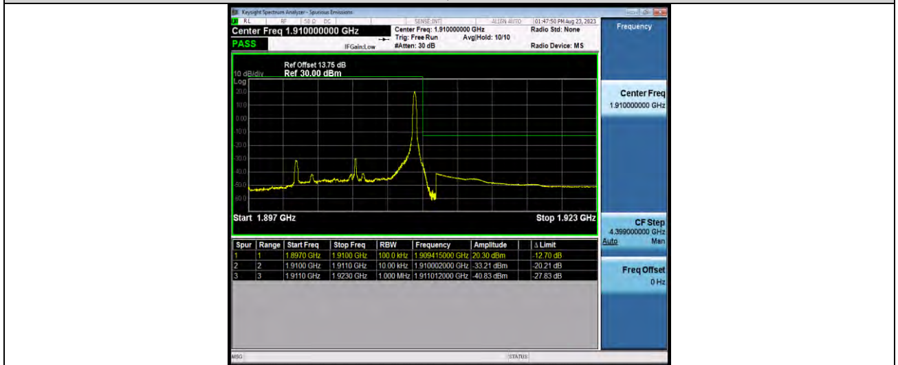
Band2-10MHz-64QAM-19150-50RB#0
