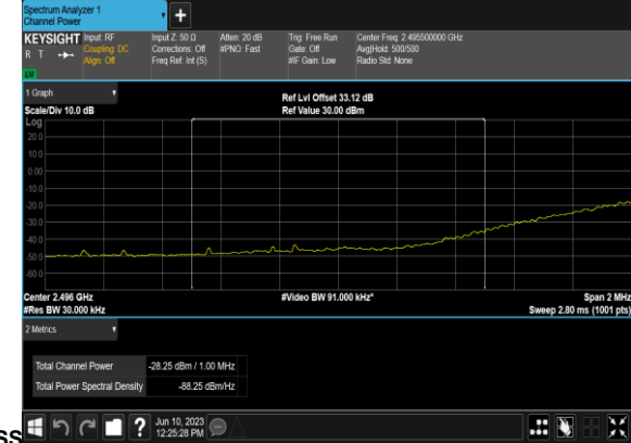
N41(100M)_DFT-s-OFDM_QPSK_Edge_1RB_Left_Low_CH_CHP_PA
