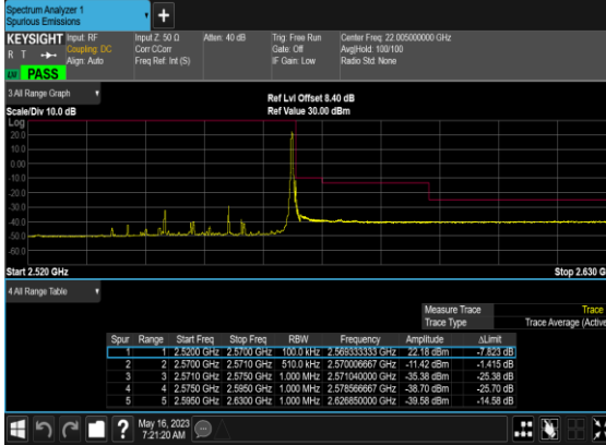
N7(25M)_DFT-s-OFDM_BPSK_Edge_1RB_Right_High_CH
