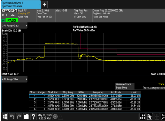
N7(25M)_DFT-s-OFDM_BPSK_Outer_Full_High_CH
