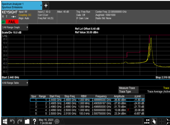
N7(50M)_DFT-s-OFDM_BPSK_Edge_1RB_Left_Low_CH
