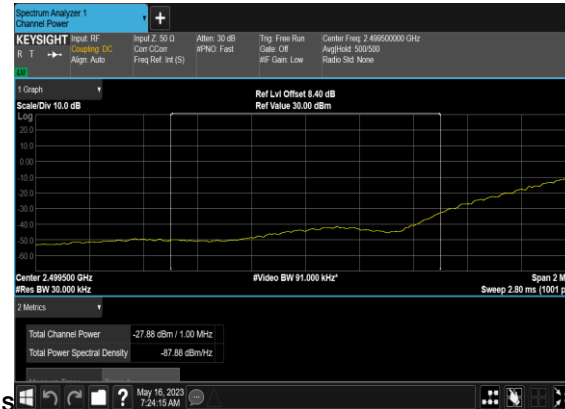
N7(50M)_DFT-s-OFDM_BPSK_Edge_1RB_Left_Low_CH_CHP_PAS
