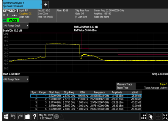
N7(25M)_DFT-s-OFDM_QPSK_Outer_Full_High_CH
