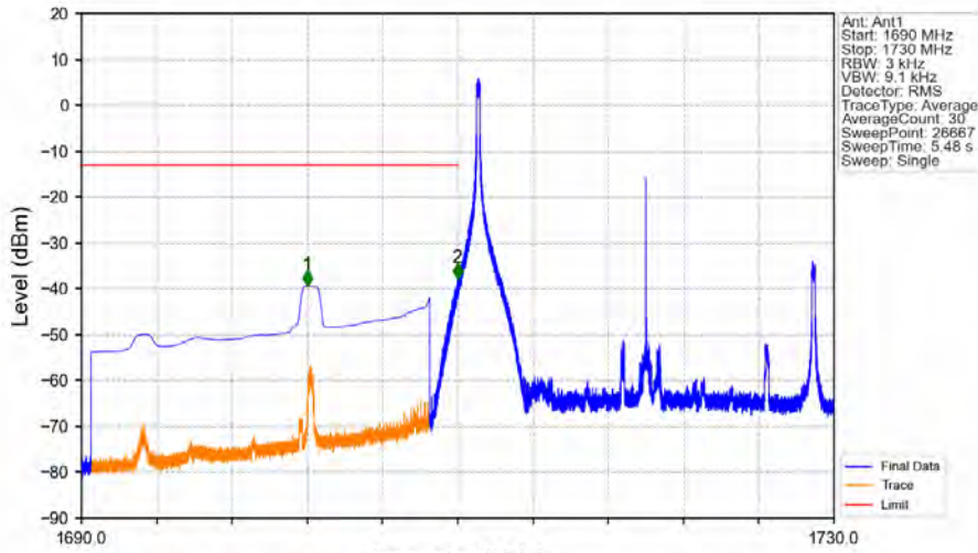
Band66_20MHz_64QAM_LCH_1720MHz_RB_1_0_NTNV
