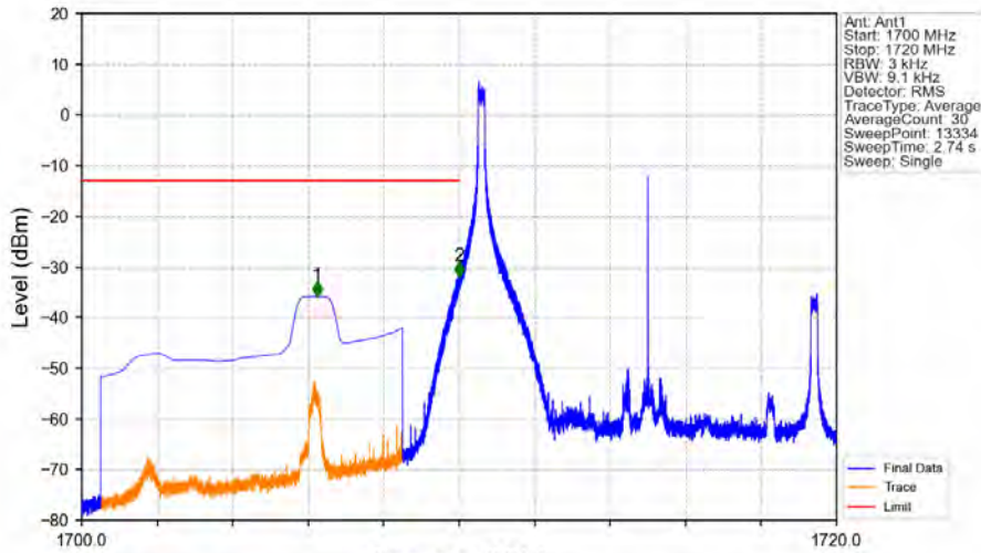
Band66_10MHz_64QAM_LCH_1715MHz_RB_1_0_NTNV
