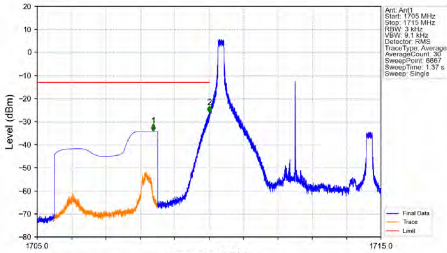
Band66_5MHz_64QAM_LCH_1712.5MHz_RB_1_0_NTNV
