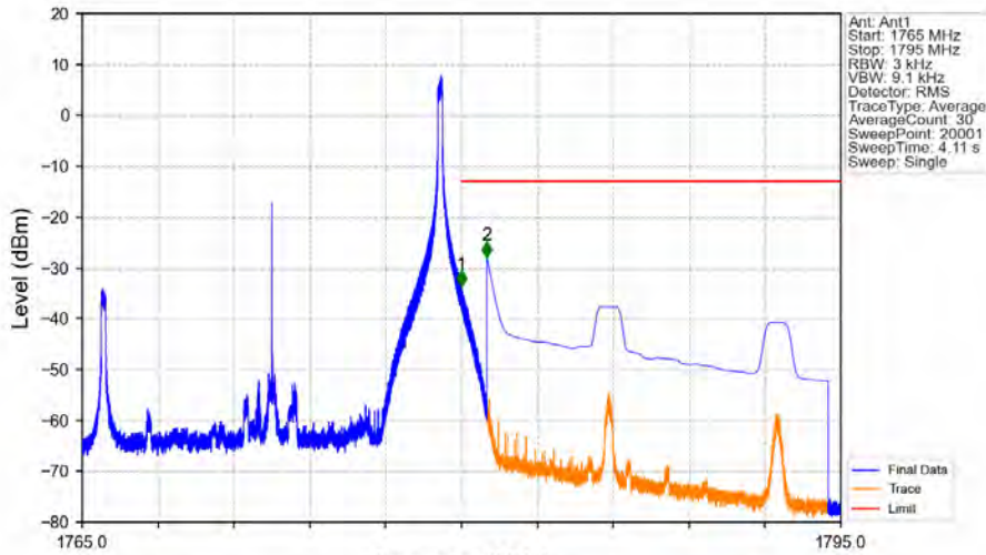
Band66_15MHz_16QAM_HCH_1772.5MHz_RB_1_74_NTNV
