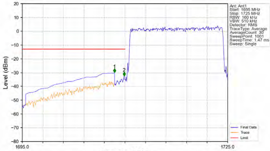
Band66_15MHz_64QAM_LCH_1717.5MHz_RB_75_0_NTNV
