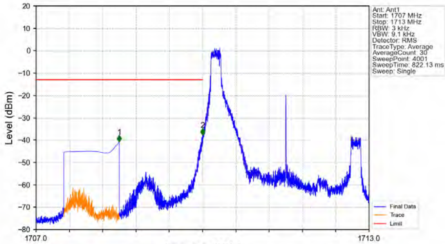
Band66_3MHz_64QAM_LCH_1711.5MHz_RB_1_0_NTNV
