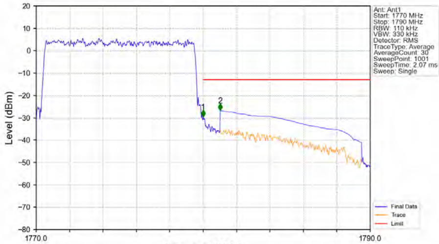
Band66_10MHz_QPSK_HCH_1775MHz_RB_50_0_NTNV
