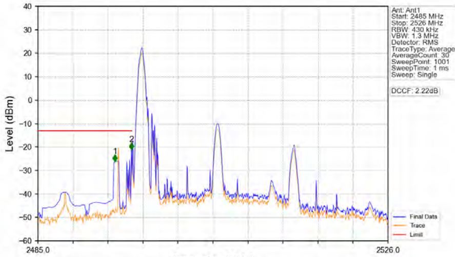
Band41_20MHz_16QAM_LCH_2506MHz_RB_1_0_NTNV
