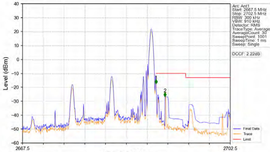
Band41_15MHz_16QAM_HCH_2682.5MHz_RB_1_74_NTNV
