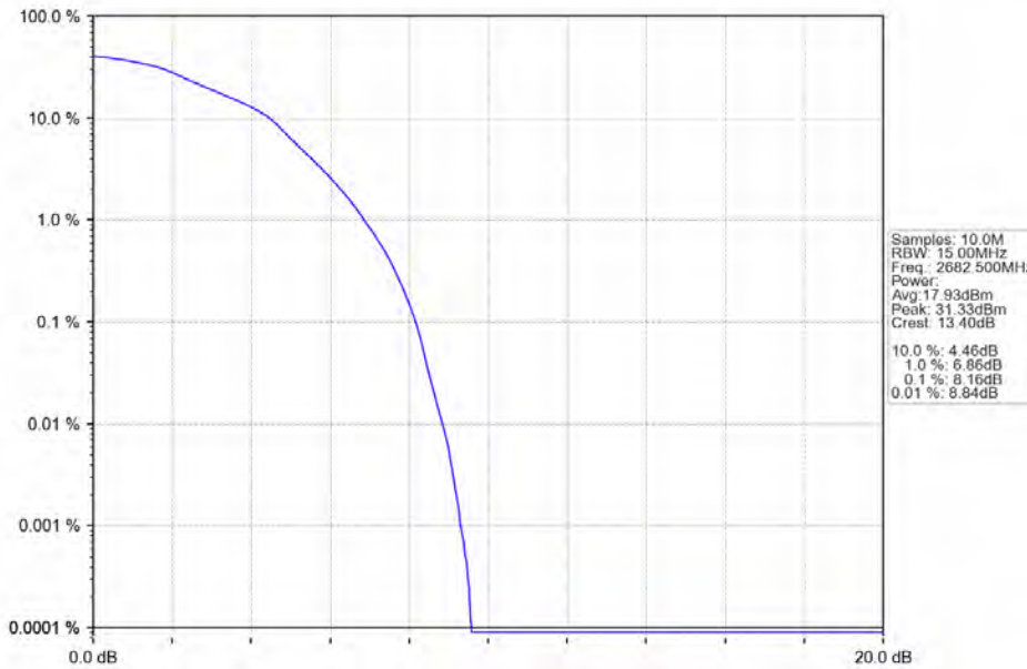
Band41_15MHz_16QAM_HCH_2682.5MHz_RB_75_0_NTNV
