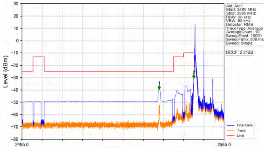
Band38_10MHz_64QAM_LCH_2575MHz_RB_1_0_NTNV
