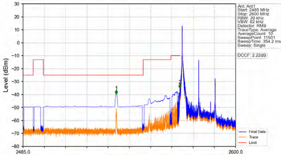
Band38_20MHz_64QAM_LCH_2580MHz_RB_1_0_NTNV
