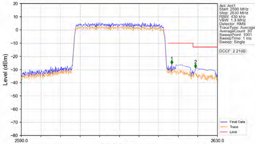
Band38_20MHz_64QAM_HCH_2610MHz_RB_100_0_NTNV
