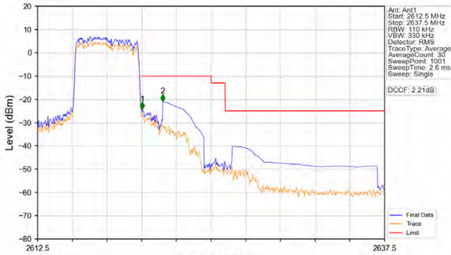
Band38_5MHz_QPSK_HCH_2617.5MHz_RB_25_0_NTNV
