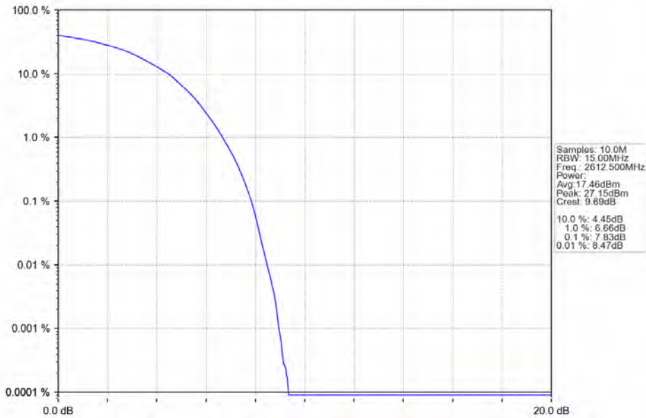
Band38_15MHz_64QAM_HCH_2612.5MHz_RB_75_0_NTNV
