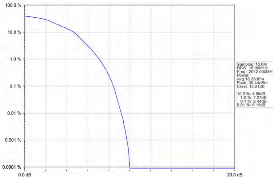
Band38_15MHz_16QAM_HCH_2612.5MHz_RB_75_0_NTNV
