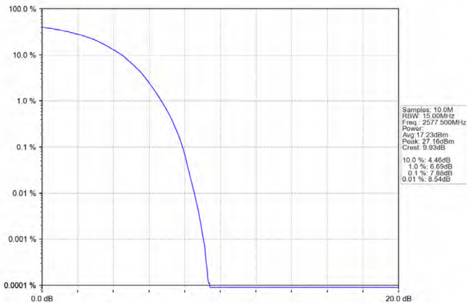
Band38_15MHz_64QAM_LCH_2577.5MHz_RB_75_0_NTNV
