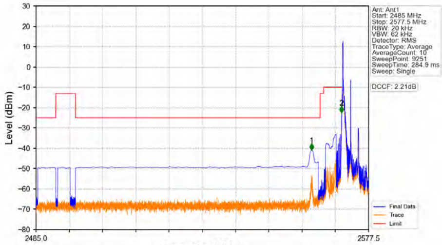
Band38_5MHz_16QAM_LCH_2572.5MHz_RB_1_0_NTNV
