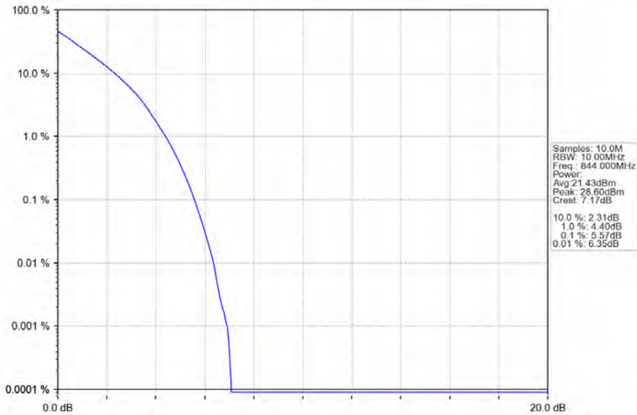
Band26b_10MHz_QPSK_HCH_844MHz_RB_50_0_NTNV
