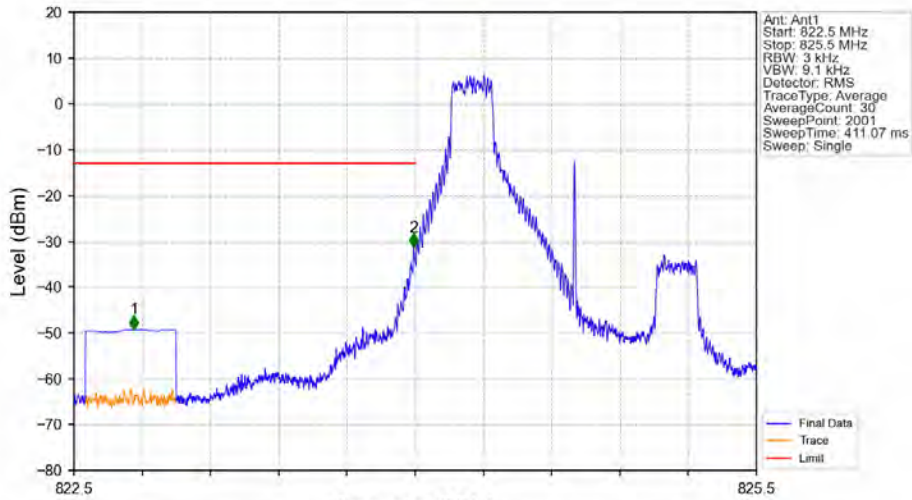
Band26b_1.4MHz_64QAM_LCH_824.7MHz_RB_1_0_NTNV
