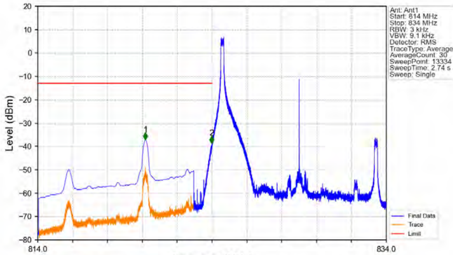
Band26b_10MHz_16QAM_LCH_829MHz_RB_1_0_NTNV
