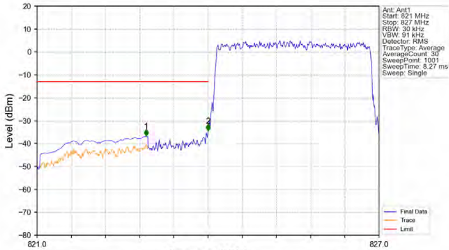
Band26b_3MHz_QPSK_LCH_825.5MHz_RB_15_0_NTV
