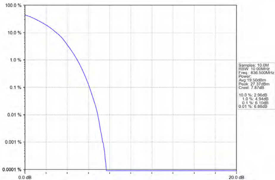
Band26b_10MHz_64QAM_MCH_836.5MHz_RB_50_0_NTNV
