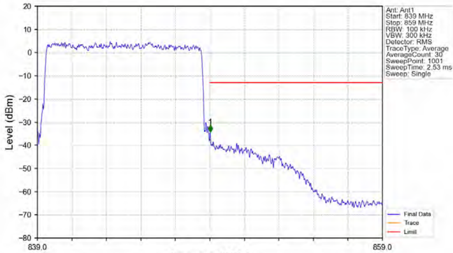
Band26b_10MHz_QPSK_HCH_844MHz_RB_50_0_NTNV
