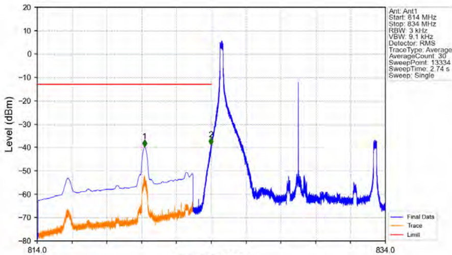
Band26b_10MHz_64QAM_LCH_829MHz_RB_1_0_NTNV
