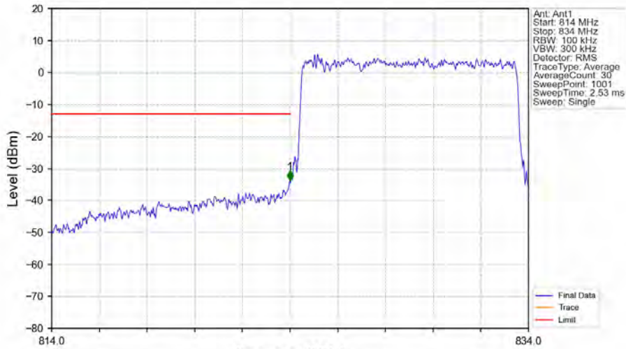
Band26b_10MHz_QPSK_LCH_829MHz_RB_50_0_NTNV
