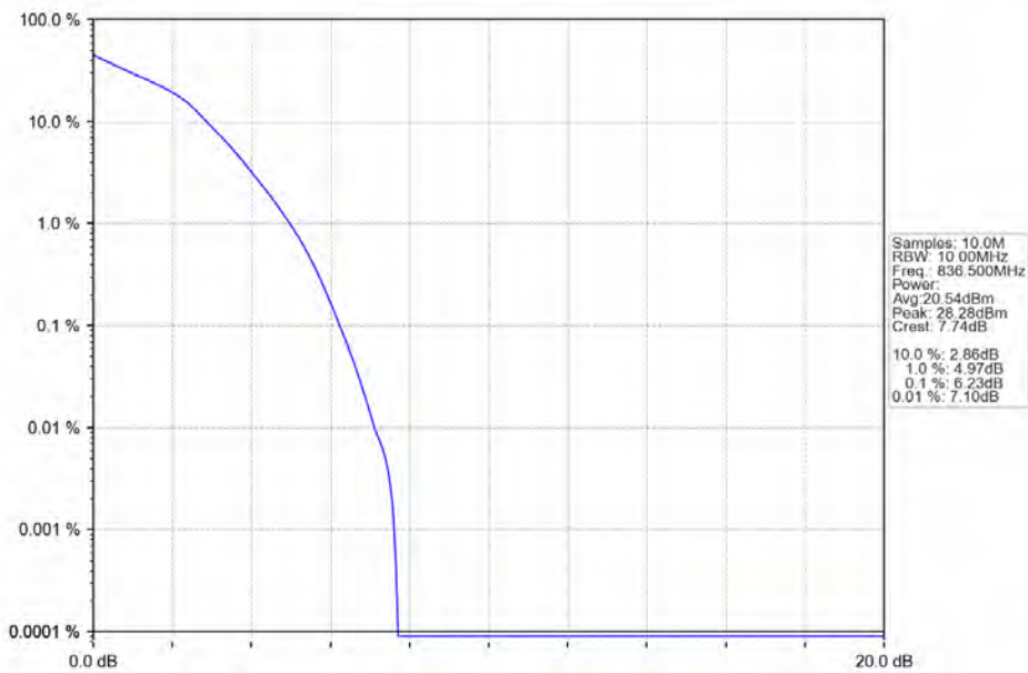
Band26b_10MHz_16QAM_MCH_836.5MHz_RB_50_0_NTNV
