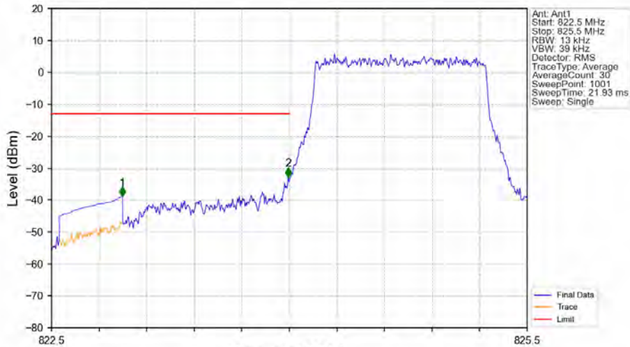
Band26b_1.4MHz_QPSK_LCH_824.7MHz_RB_6_0_NTNV
