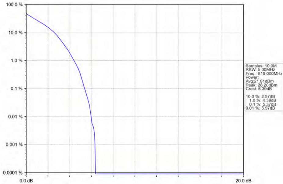
Band26a_1.4MHz_QPSK_MCH_819MHz_RB_6_0_NTNV
