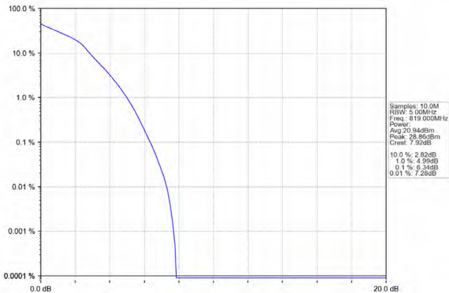
Band26a_5MHz_16QAM_MCH_819MHz_RB_25_0_NTNV
