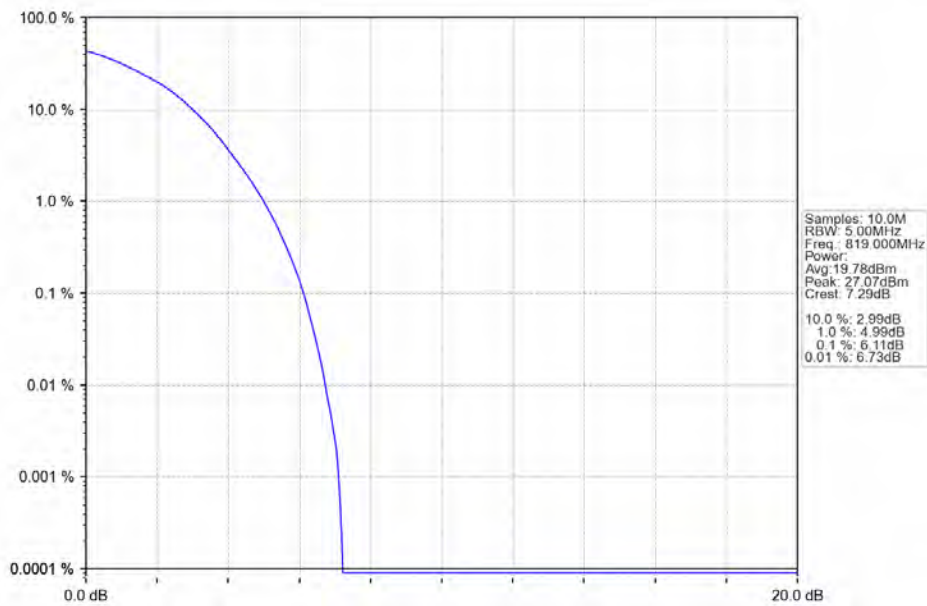
Band26a_3MHz_64QAM_MCH_819MHz_RB_15_0_NTNV
