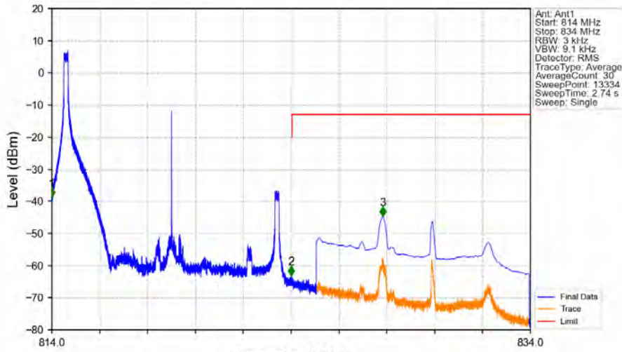
Band26a_10MHz_16QAM_MCH_819MHz_RB_1_0_NTNV
