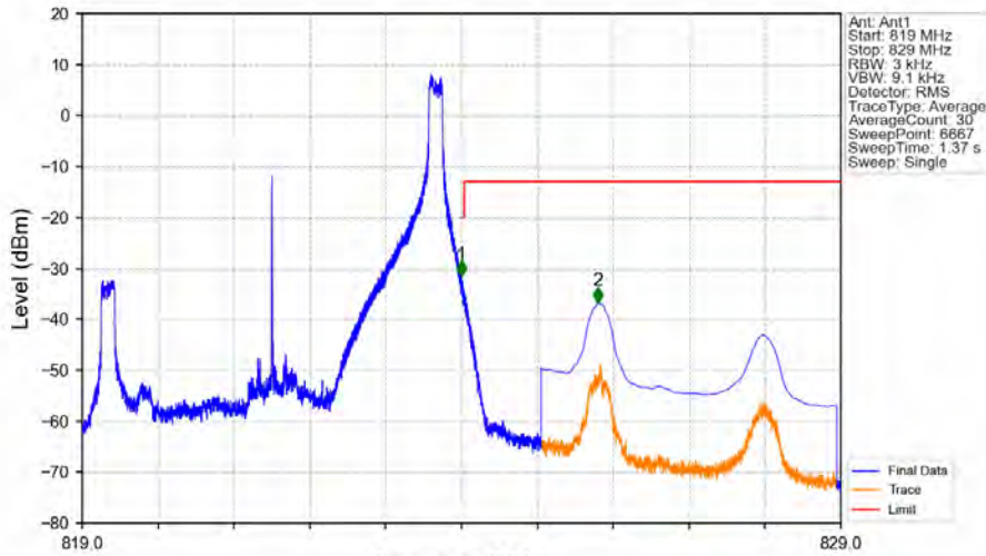
Band26a_5MHz_QPSK_HCH_821.5MHz_RB_1_24_NTNV
