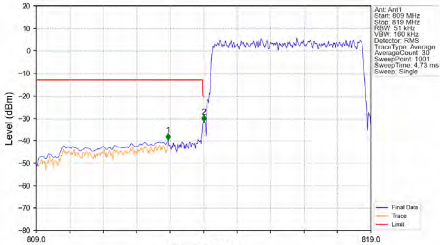
Band26a_5MHz_QPSK_LCH_816.5MHz_RB_25_0_NTNV
