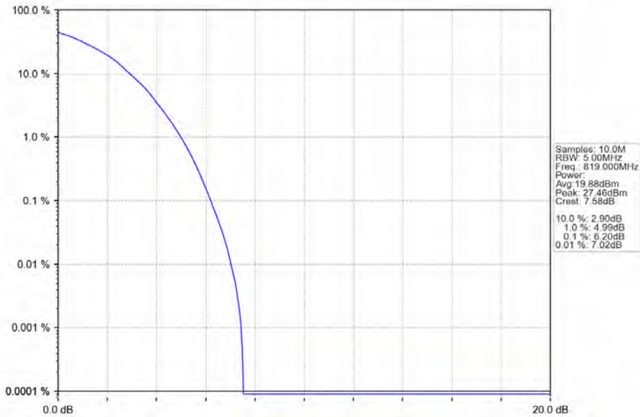
Band26a_5MHz_64QAM_MCH_819MHz_RB_25_0_NTNV
