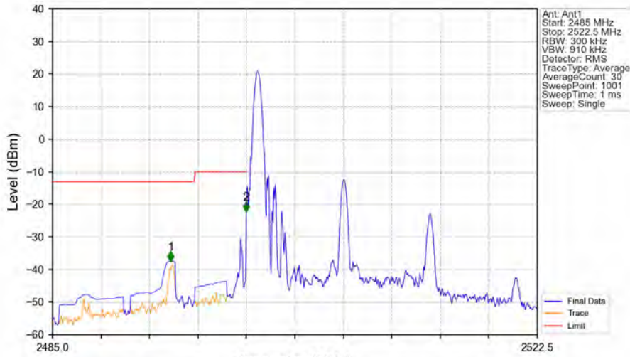
Band7_15MHz_64QAM_LCH_2507.5MHz_RB_1_0_NTNV
