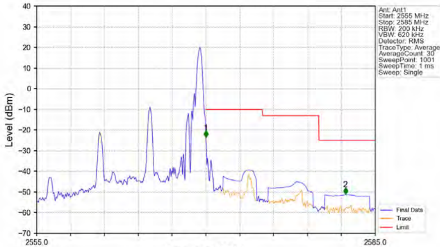
Band7_10MHz_64QAM_HCH_2565MHz_RB_1_49_NTNV
