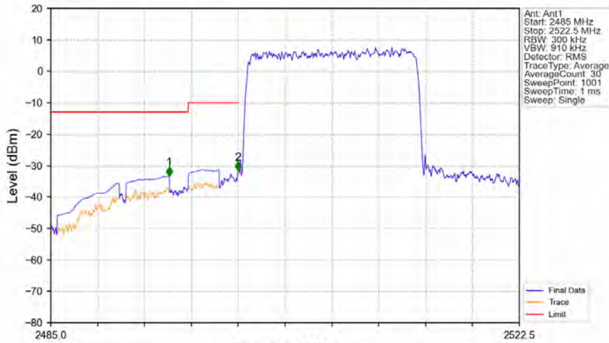
Band7_15MHz_QPSK_LCH_2507.5MHz_RB_75_0_NTNV
