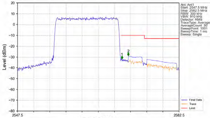
Band7_15MHz_QPSK_HCH_2562.5MHz_RB_75_0_NTNV
