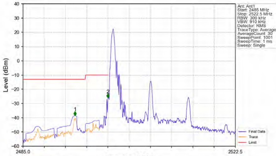
Band7_15MHz_16QAM_LCH_2507.5MHz_RB_1_0_NTNV
