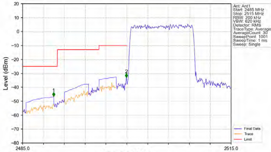
Band7_10MHz_64QAM_LCH_2505MHz_RB_50_0_NTNV
