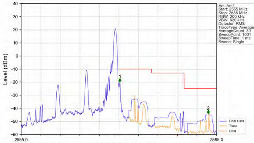
Band7_10MHz_16QAM_HCH_2565MHz_RB_1_49_NTNV
