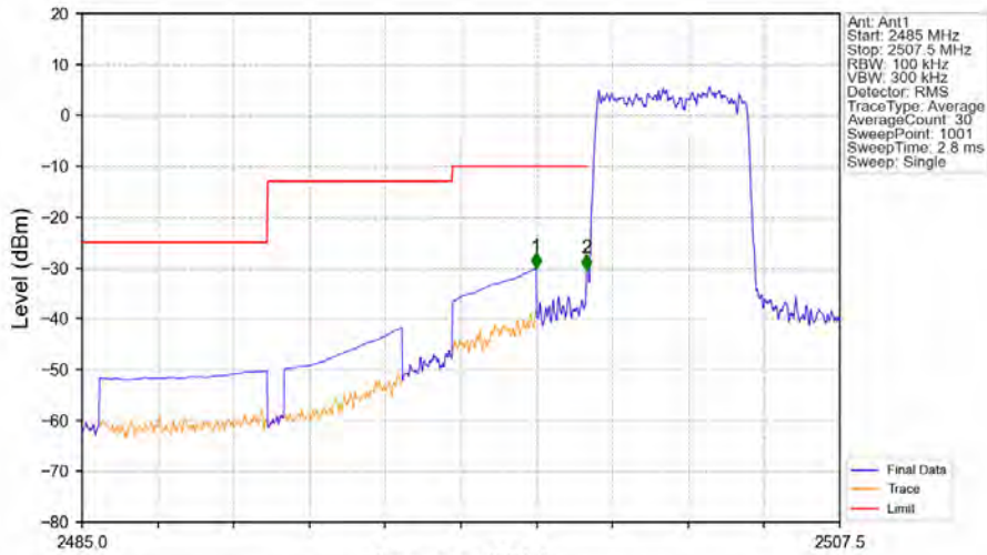
Band7_5MHz_64QAM_LCH_2502.5MHz_RB_25_0_NTNV
