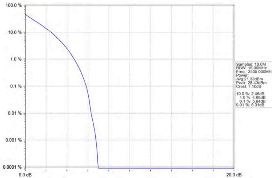
Band7_15MHz_QPSK_MCH_2535MHz_RB_75_0_NTNV
