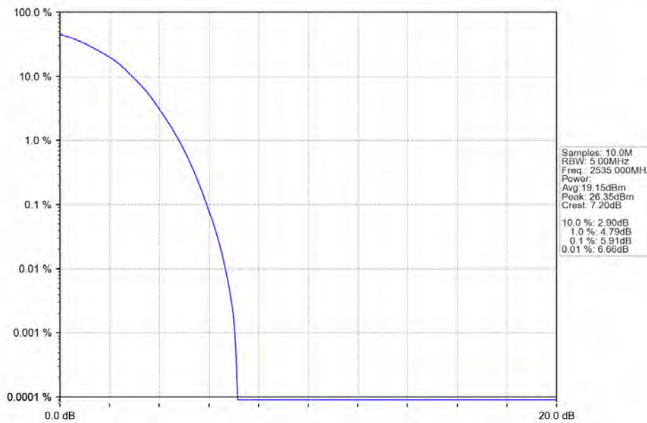
Band7_5MHz_64QAM_MCH_2535MHz_RB_25_0_NTNV
