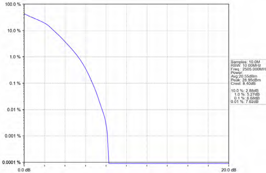
Band7_10MHz_16QAM_LCH_2505MHz_RB_50_0_NTNV
