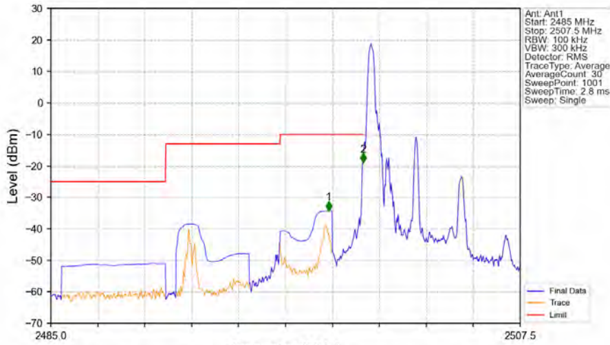
Band7_5MHz_16QAM_LCH_2502.5MHz_RB_1_0_NTNV
