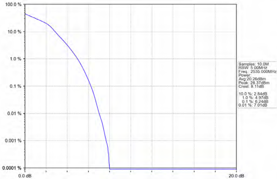
Band7_5MHz_16QAM_MCH_2535MHz_RB_25_0_NTNV
