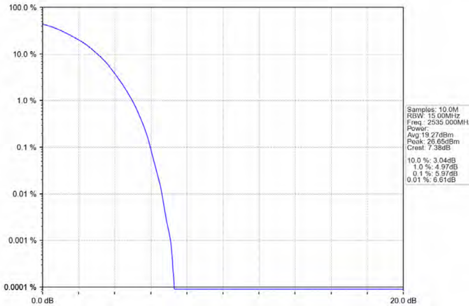
Band7_15MHz_64QAM_MCH_2535MHz_RB_75_0_NTNV
