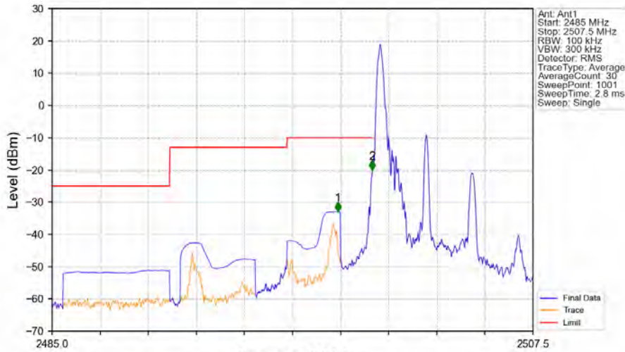
Band7_5MHz_64QAM_LCH_2502.5MHz_RB_1_0_NTNV
