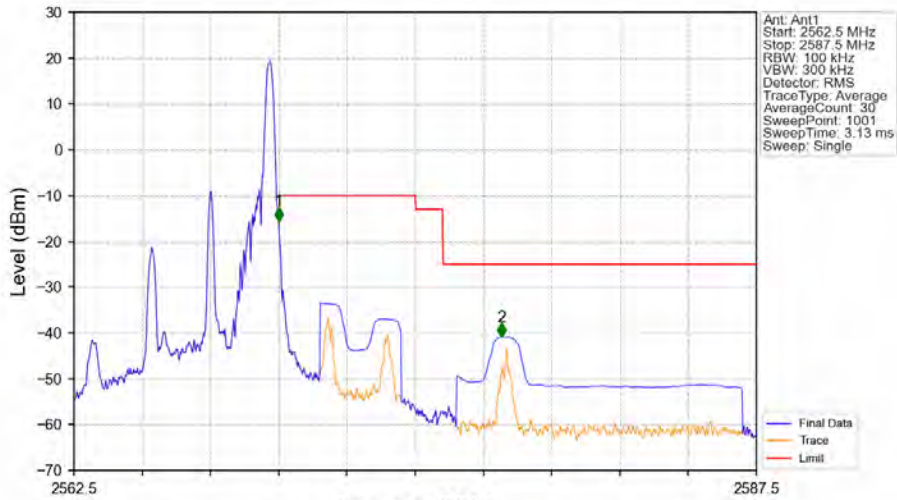
Band7_5MHz_16QAM_HCH_2567.5MHz_RB_1_24_NTNV
