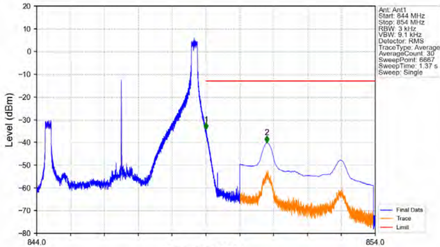
Band5_5MHz_16QAM_HCH_846.5MHz_RB_1_24_NTNV
