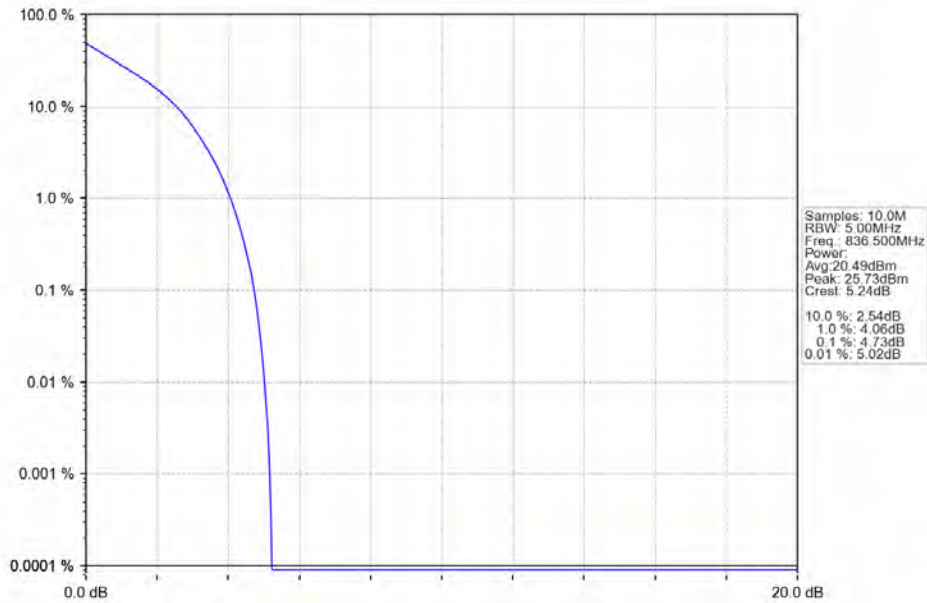
Band5_1.4MHz_QPSK_MCH_836.5MHz_RB_6_0_NTNV
