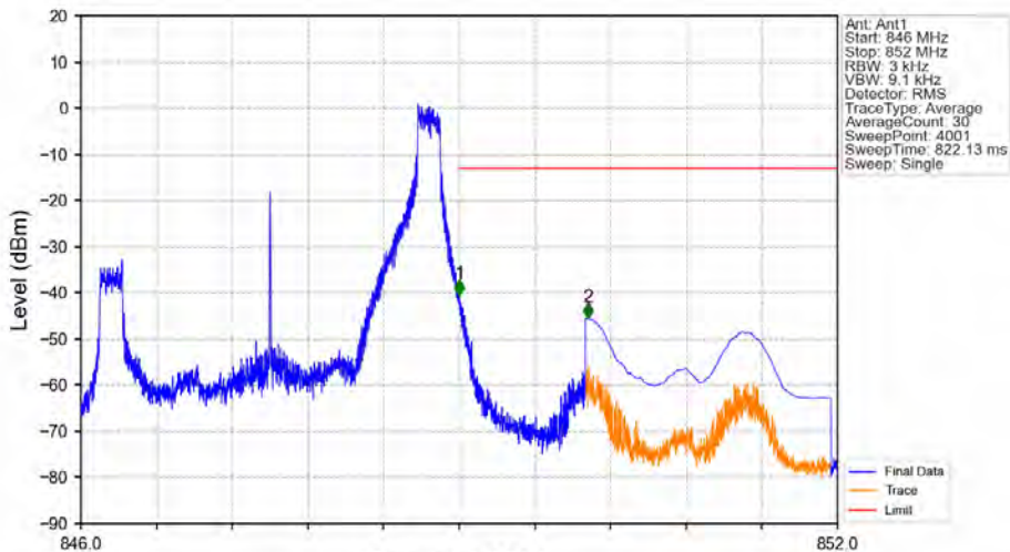
Band5_3MHz_64QAM_HCH_847.5MHz_RB_1_14_NTNV
