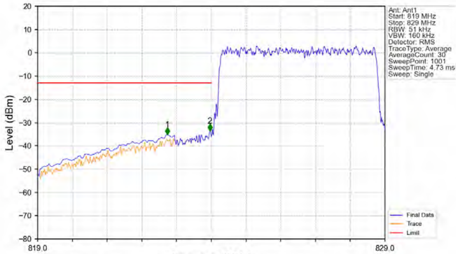
Band5_5MHz_64QAM_LCH_826.5MHz_RB_25_0_NTNV
