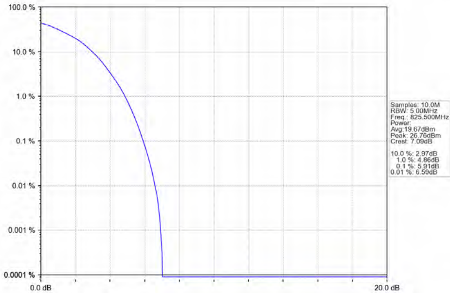
Band5_3MHz_64QAM_LCH_825.5MHz_RB_15_0_NTNV
