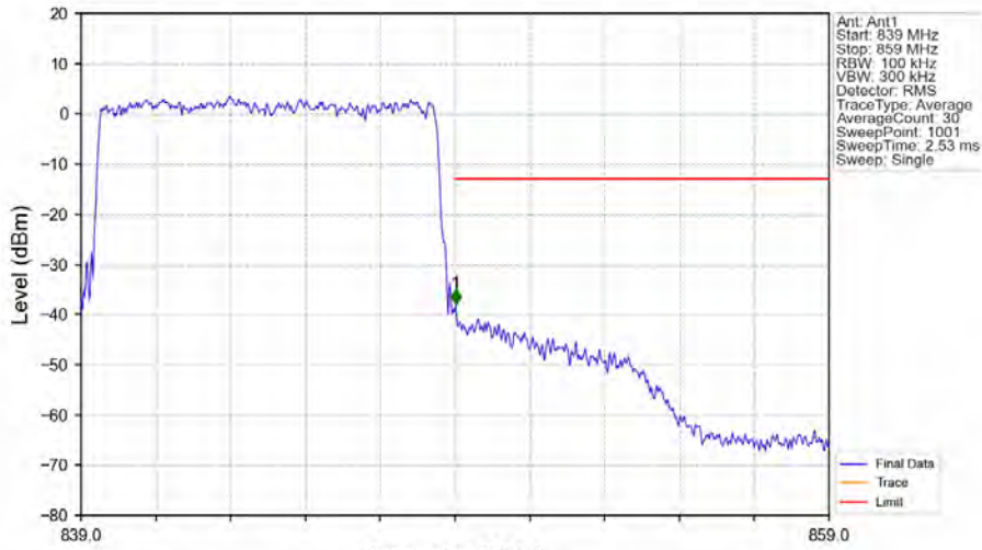
Band5_10MHz_16QAM_HCH_844MHz_RB_50_0_NTNV
