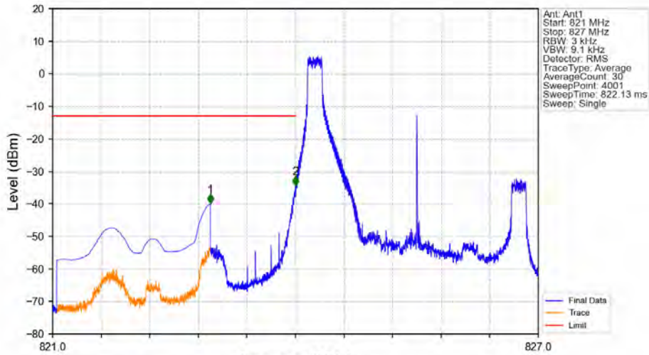
Band5_3MHz_64QAM_LCH_825.5MHz_RB_1_0_NTNV
