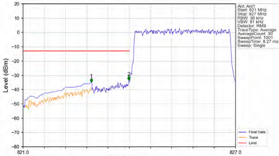
Band5_3MHz_64QAM_LCH_825.5MHz_RB_15_0_NTNV
