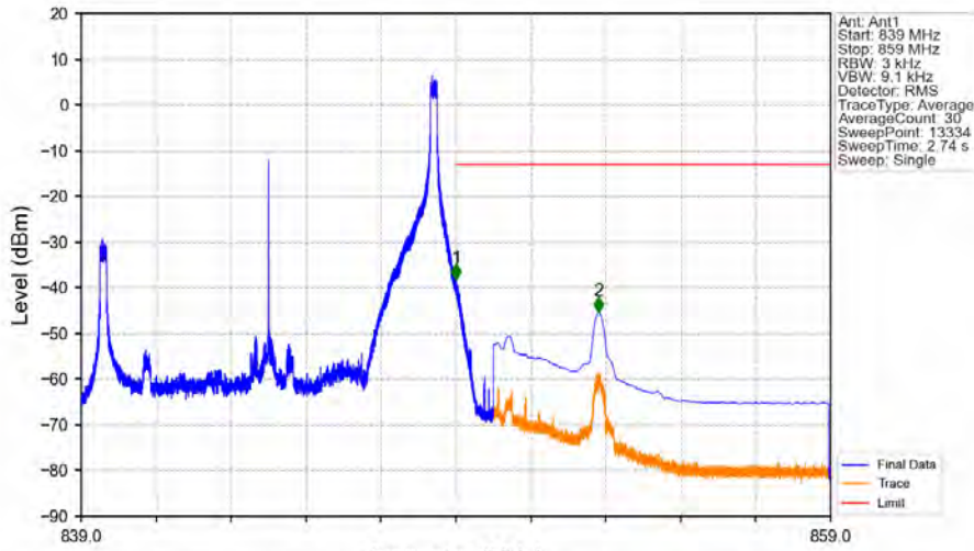
Band5_10MHz_16QAM_HCH_844MHz_RB_1_49_NTNV
