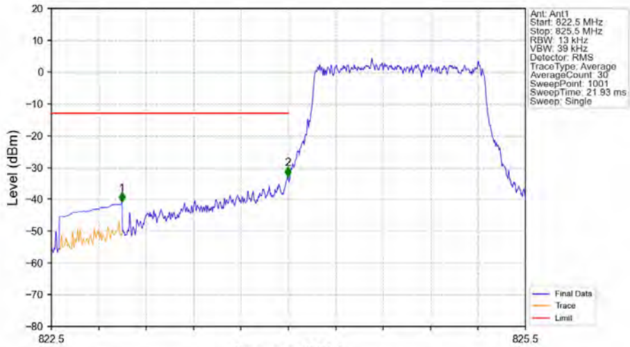
Band5_1.4MHz_64QAM_LCH_824.7MHz_RB_6_0_NTNV
