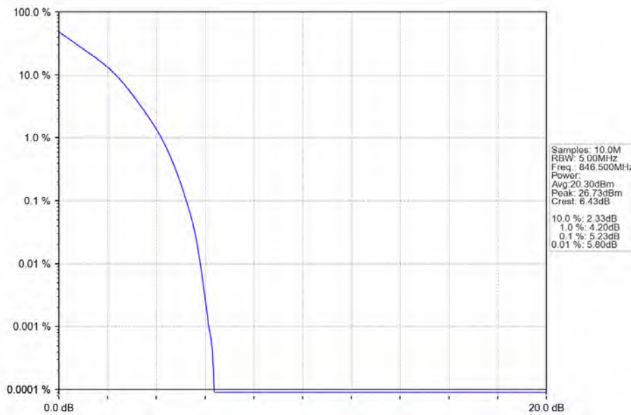
Band5_5MHz_QPSK_HCH_846.5MHz_RB_25_0_NTNV
