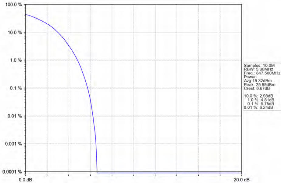
Band5_3MHz_64QAM_HCH_847.5MHz_RB_15_0_NTNV
