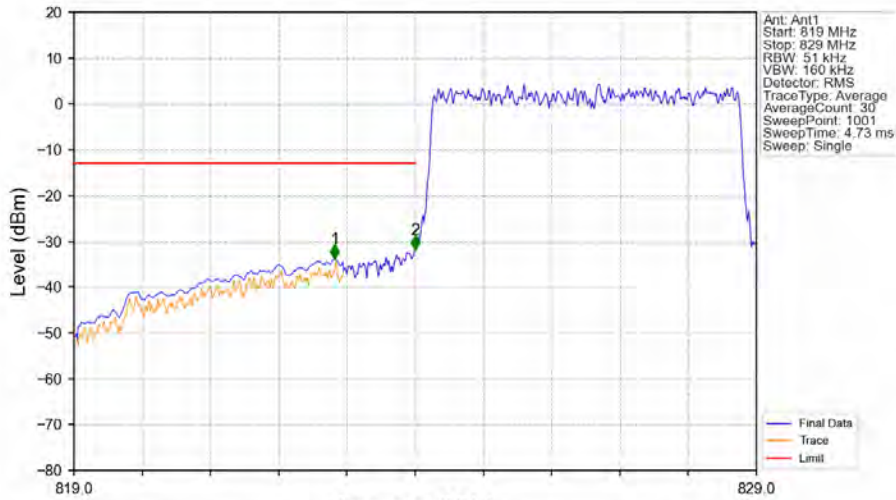
Band5_5MHz_QPSK_LCH_826.5MHz_RB_25_0_NTNV
