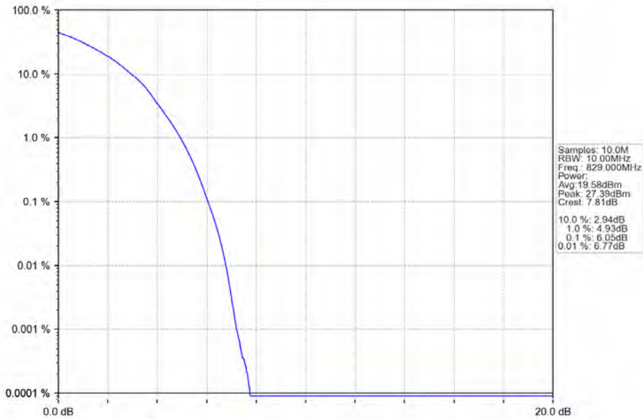
Band5_10MHz_64QAM_LCH_829MHz_RB_50_0_NTNV
