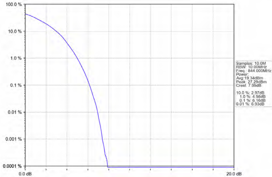
Band5_10MHz_64QAM_HCH_844MHz_RB_50_0_NTNV
