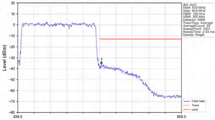
Band5_10MHz_64QAM_HCH_844MHz_RB_50_0_NTNV
