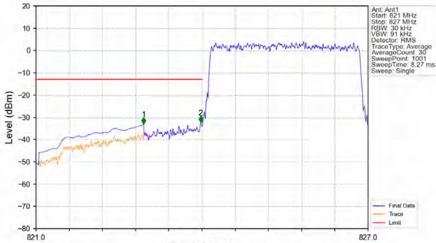
Band5_3MHz_QPSK_LCH_825.5MHz_RB_15_0_NTNV
