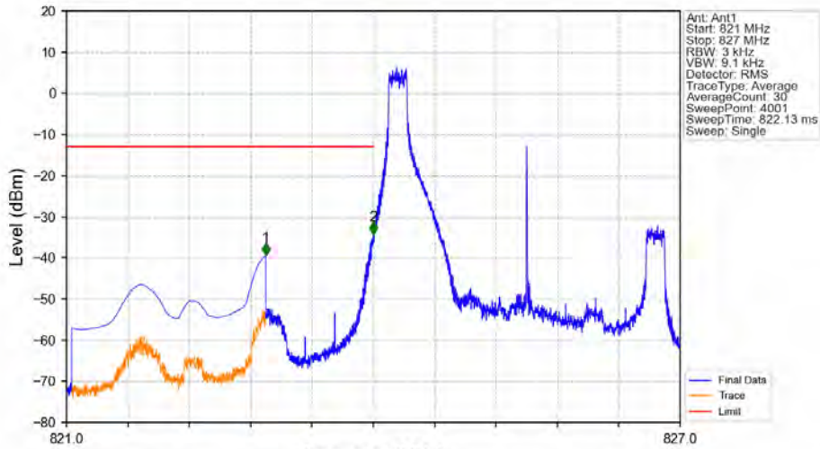
Band5_3MHz_16QAM_LCH_825.5MHz_RB_1_0_NTNV
