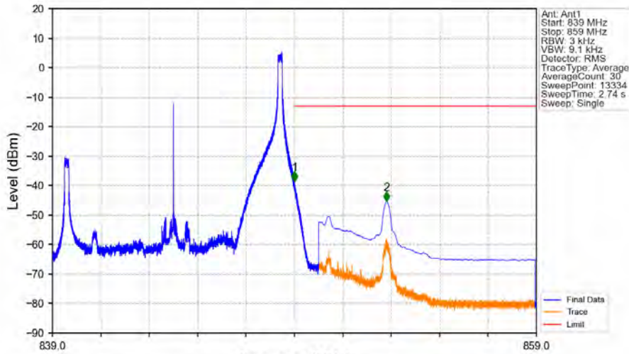
Band5_10MHz_64QAM_HCH_844MHz_RB_1_49_NTNV
