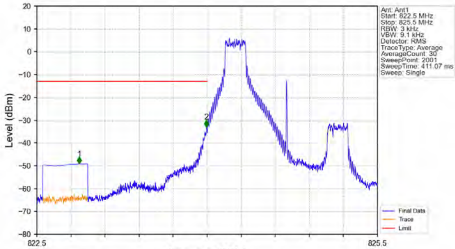
Band5_1.4MHz_64QAM_LCH_824.7MHz_RB_1_0_NTNV
