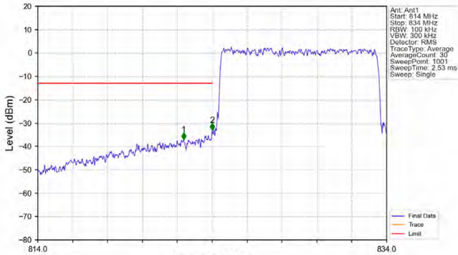
Band5_10MHz_64QAM_LCH_829MHz_RB_50_0_NTNV
