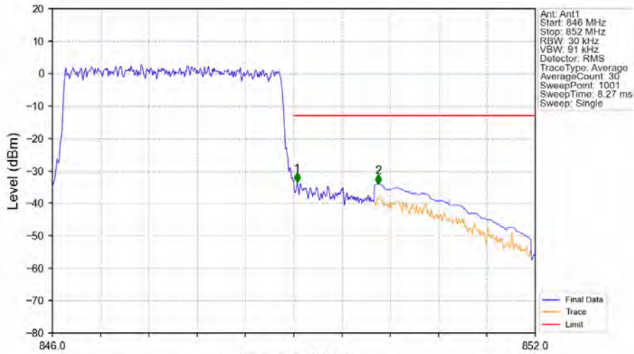
Band5_3MHz_64QAM_HCH_847.5MHz_RB_15_0_NTNV
