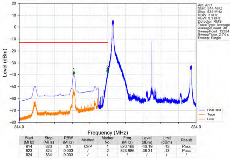
Band5_10MHz_64QAM_LCH_829MHz_RB_1_0_NTNV
