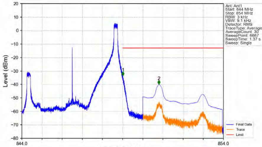
Band5_5MHz_64QAM_HCH_846.5MHz_RB_1_24_NTNV
