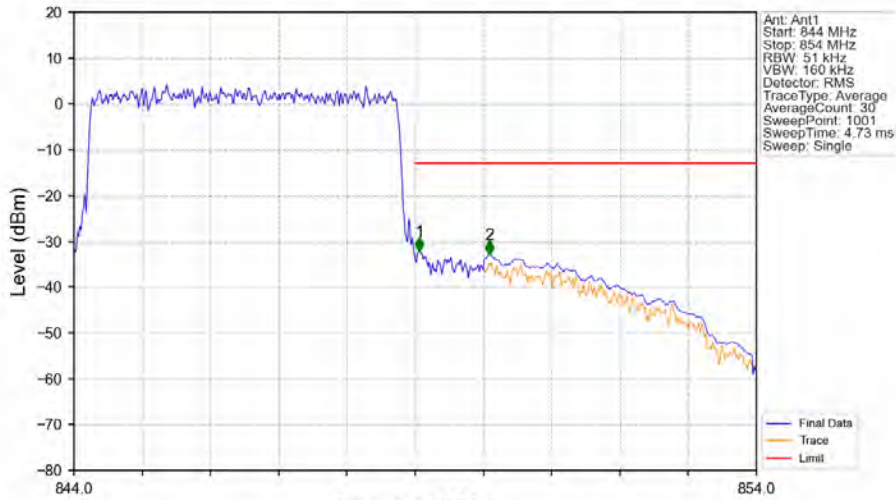
Band5_5MHz_QPSK_HCH_846.5MHz_RB_25_0_NTNV
