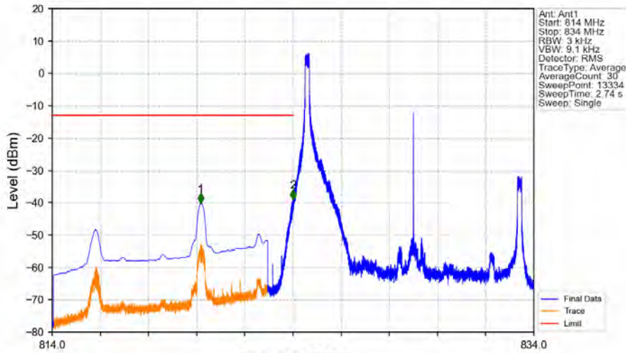
Band5_10MHz_16QAM_LCH_829MHz_RB_1_0_NTNV
