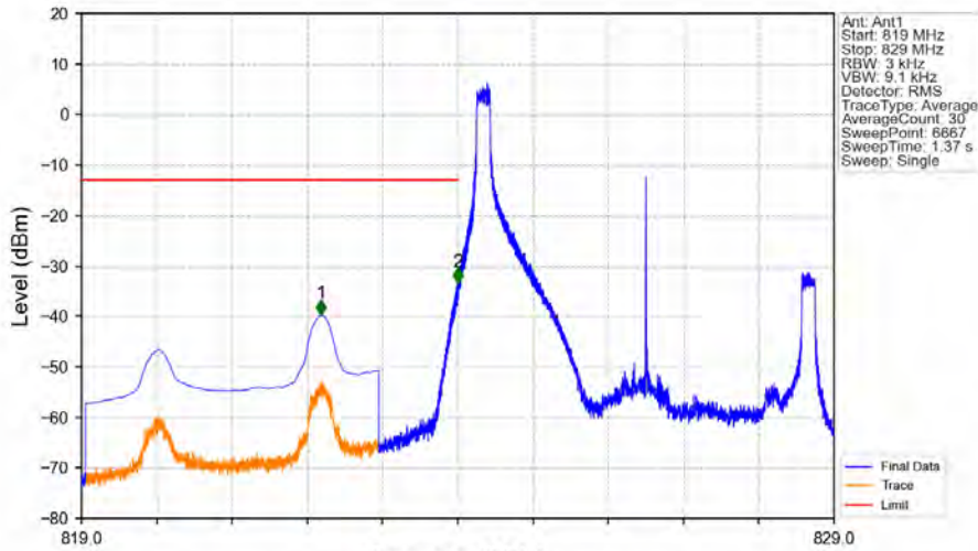
Band5_5MHz_16QAM_LCH_826.5MHz_RB_1_0_NTNV
