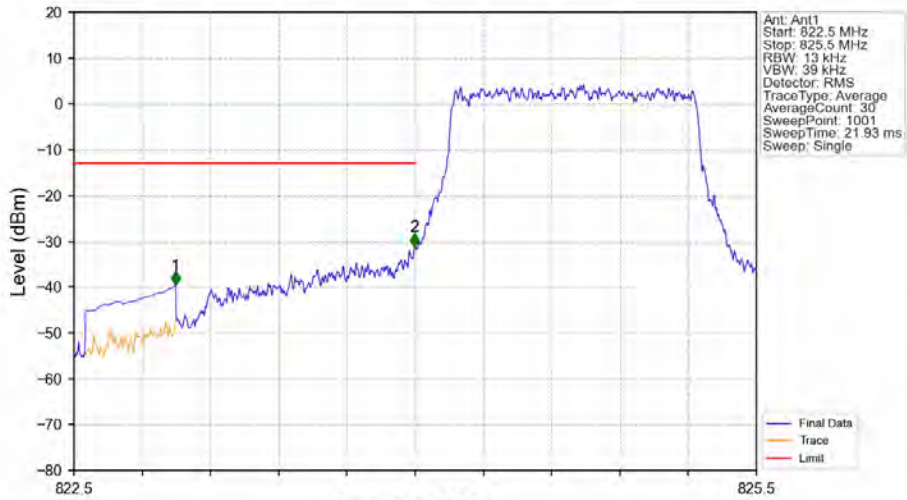
Band5_1.4MHz_QPSK_LCH_824.7MHz_RB_6_0_NTNV
