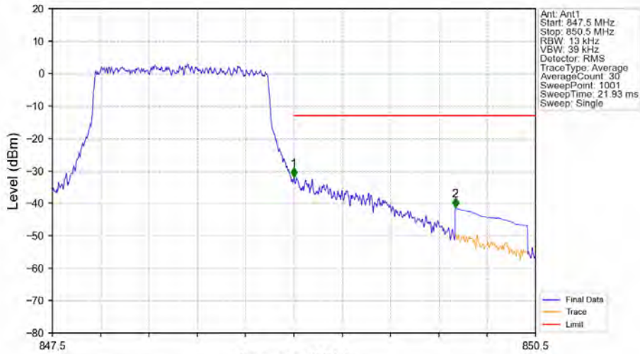
Band5_1.4MHz_64QAM_HCH_848.3MHz_RB_6_0_NTNV
