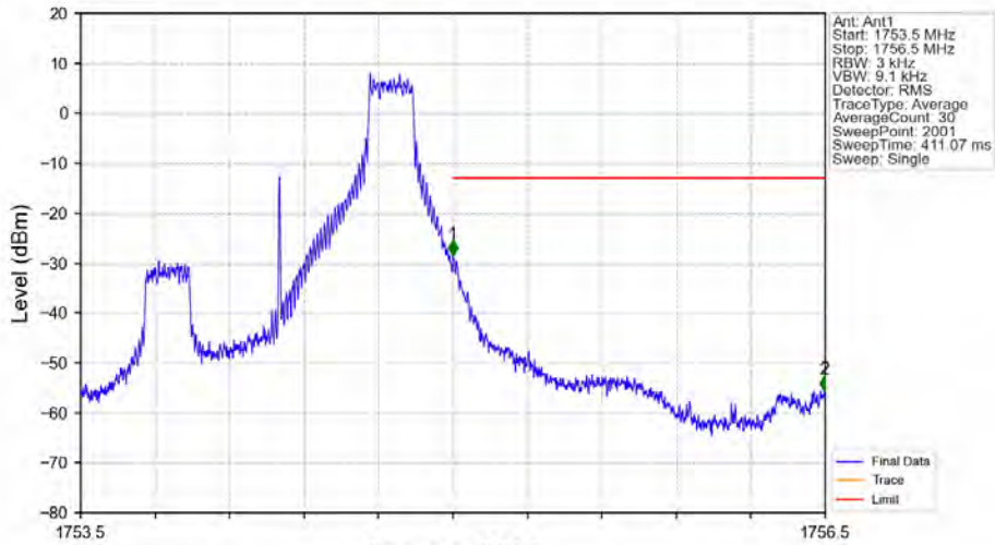
Band4 1.4MHz QPSK HCH 1754.3MHz RB 1 5 NTNV
