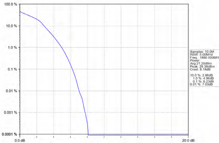
Band2_5MHz_16QAM_MCH_1880MHz_RB_25_0_NTNV
