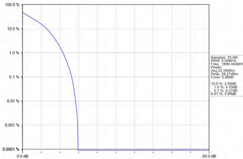
Band2_1.4MHz_QPSK_MCH_1880MHz_RB_6_0_NTNV
