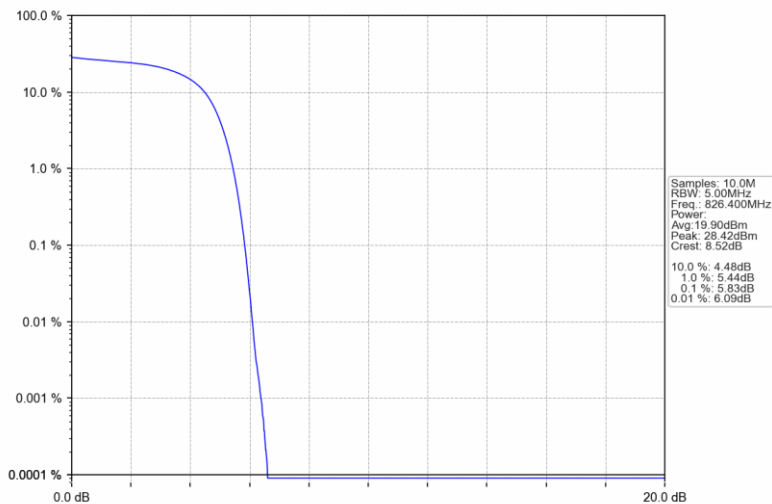
BandV_HSUPA_LCH_826.4MHz_Subtest 1_NTNV
