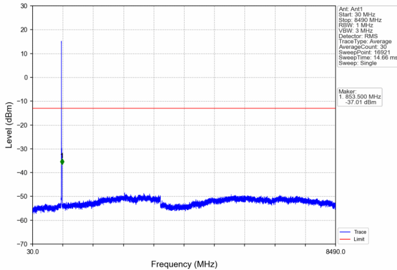
BandV_HSUPA_HCH_846.6MHz_Subtest 1_NTNV
