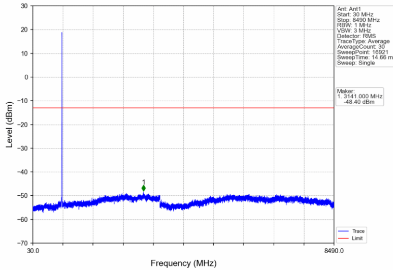
BandV_HSDPA_LCH_826.4MHz_Subtest 1_NTNV
