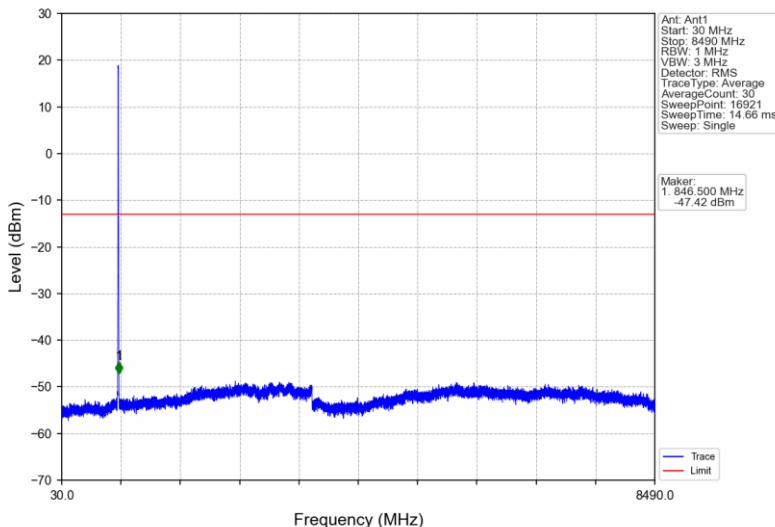
BandV_RMC_HCH_846.6MHz_12.2kbps RMC_NTNV
