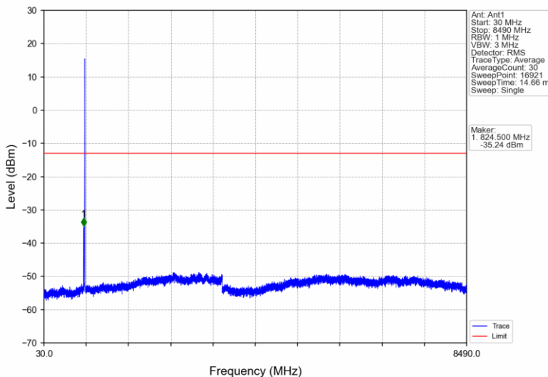
BandV_HSDPA_HCH_846.6MHz_Subtest 1_NTNV
