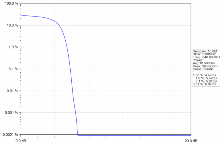
BandV_HSUPA_HCH_846.6MHz_Subtest 1_NTNV
