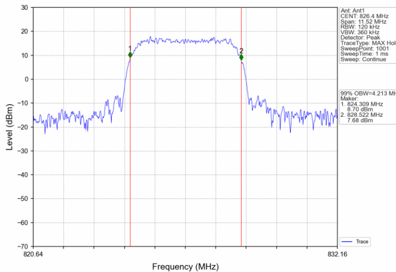
BandV_HSDPA_LCH_826.4MHz_Subtest 1_NTNV
