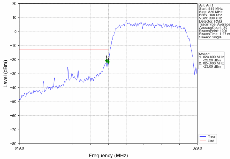
BandV_HSUPA_LCH_826.4MHz_Subtest 1_NTNV
