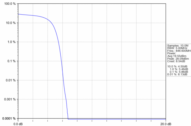
BandV_HSDPA_HCH_846.6MHz_Subtest 1_NTNV
