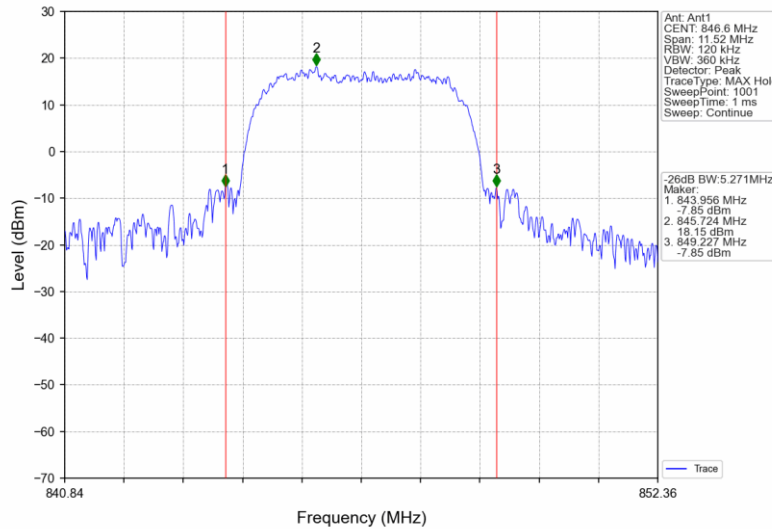
BandV_HSUPA_HCH_846.6MHz_Subtest 1_NTNV
