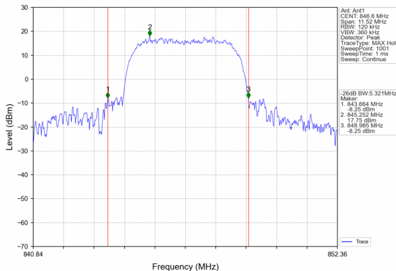
BandV_HSDPA_HCH_846.6MHz_Subtest 1_NTNV
