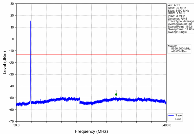
BandV_HSUPA_LCH_826.4MHz_Subtest 1_NTNV
