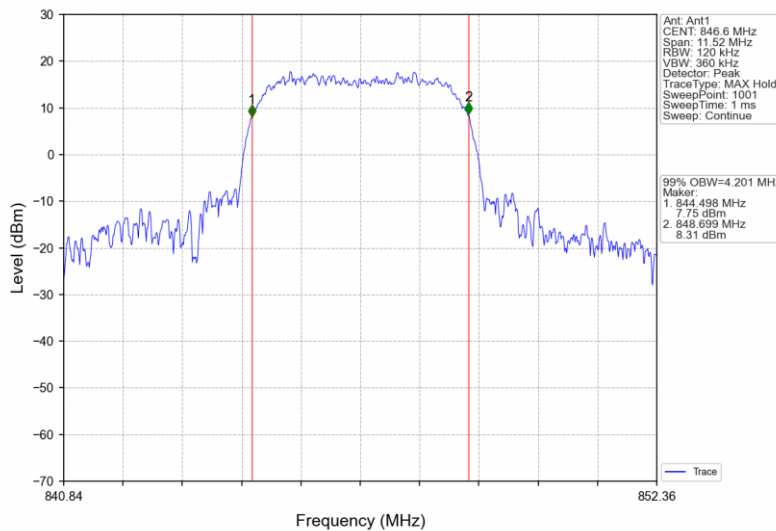
BandV_HSDPA_HCH_846.6MHz_Subtest 1_NTNV
