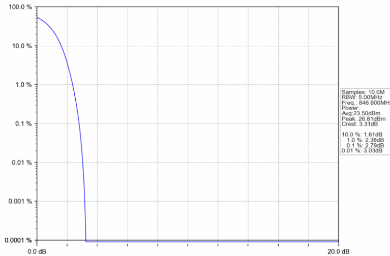
BandV_RMC_HCH_846.6MHz_12.2kbps RMC_NTNV
