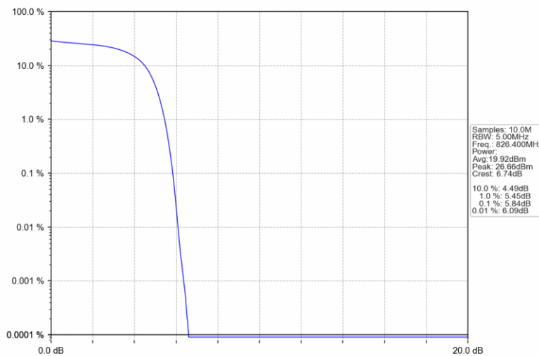
BandV_HSDPA_LCH_826.4MHz_Subtest 1_NTNV
