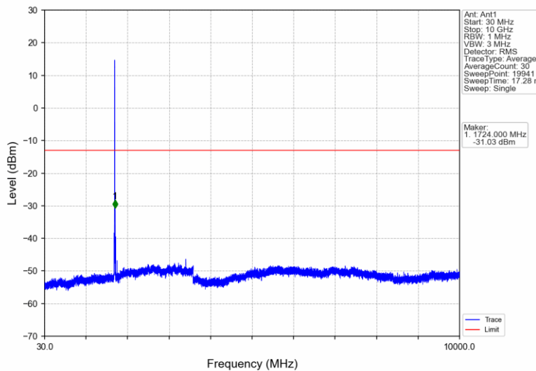
Band IV_HSDPA_LCH_1712.4MHz_Subtest 1_NTNV
