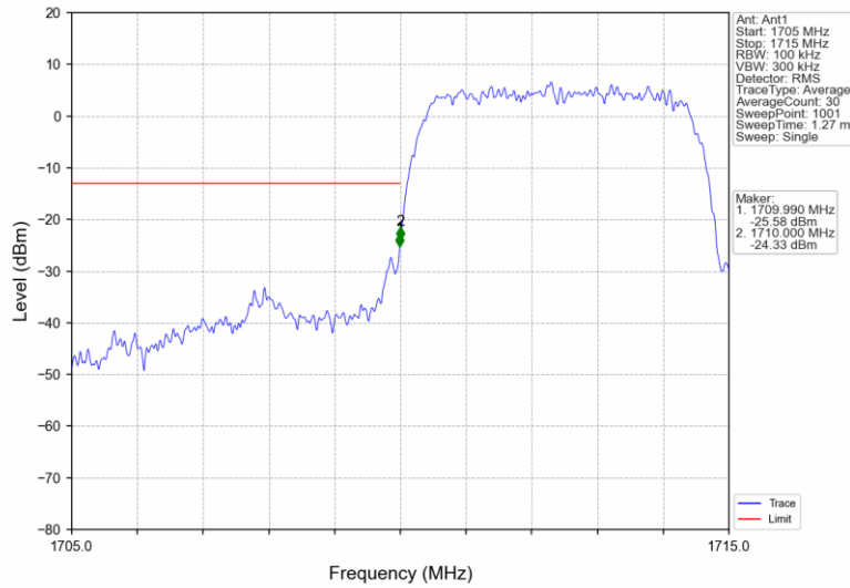
Band IV_HSUPA_LCH_1712.4MHz_Subtest 1_NTNV
