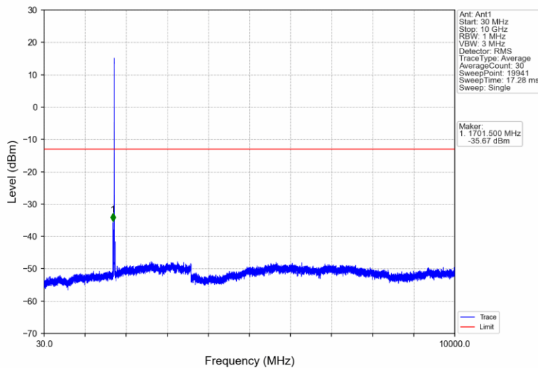
Band IV_HSDPA_MCH_1732.6MHz_Subtest 1_NTNV
