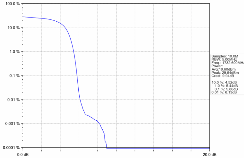
Band IV_HSDPA_MCH_1732.6MHz_Subtest 1_NTNV
