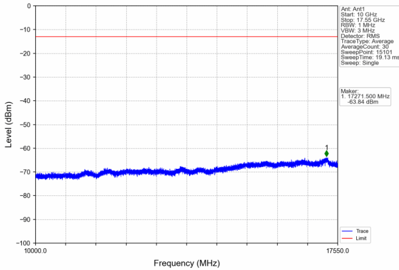
Band IV_HSUPA_HCH_1752.6MHz_Subtest 1_NTNV
