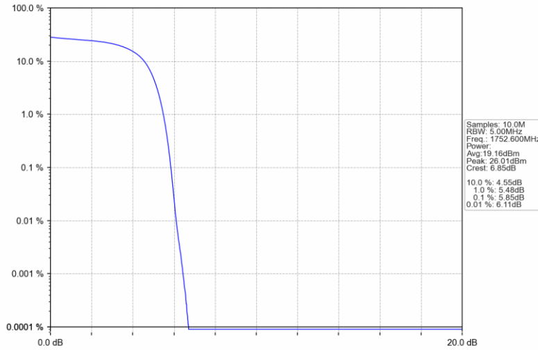
Band IV_HSUPA_HCH_1752.6MHz_Subtest 1_NTNV
