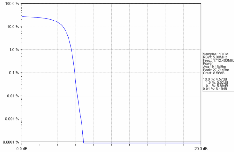
Band IV_HSUPA_LCH_1712.4MHz_Subtest 1_NTNV
