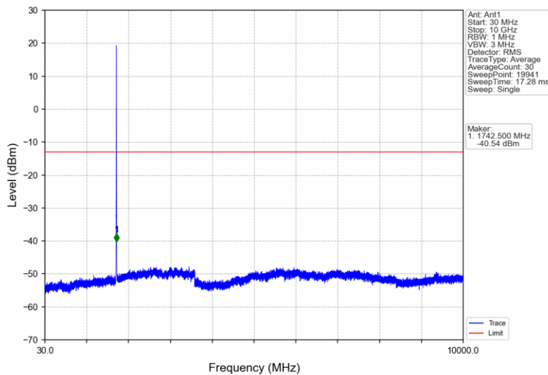
Band IV_RMC_MCH_1732.6MHz_12.2kbps RMC_NTNV
