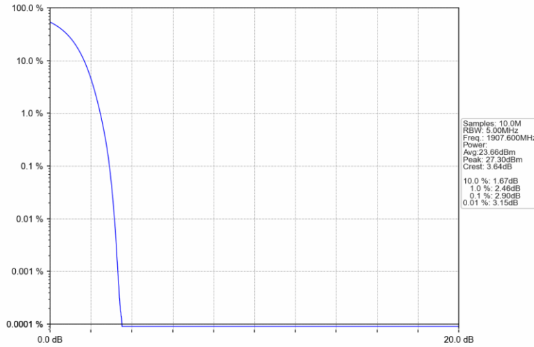
BandII_RMC_HCH_1907.6MHz_12.2kbps RMC_NTNV
