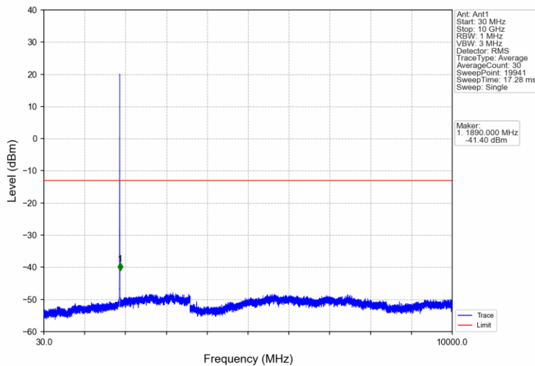
BandII_RMC_MCH_1880MHz_12.2kbps RMC_NTNV
