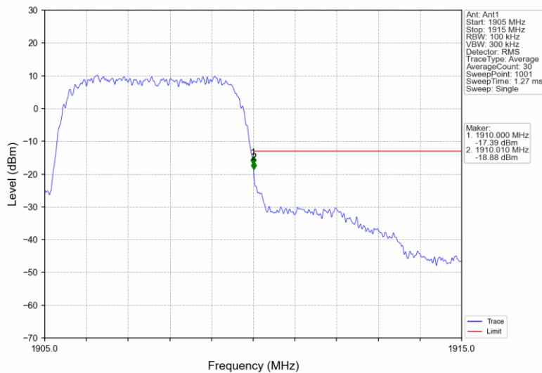
BandII_RMC_HCH_1907.6MHz_12.2kbps RMC_NTNV
