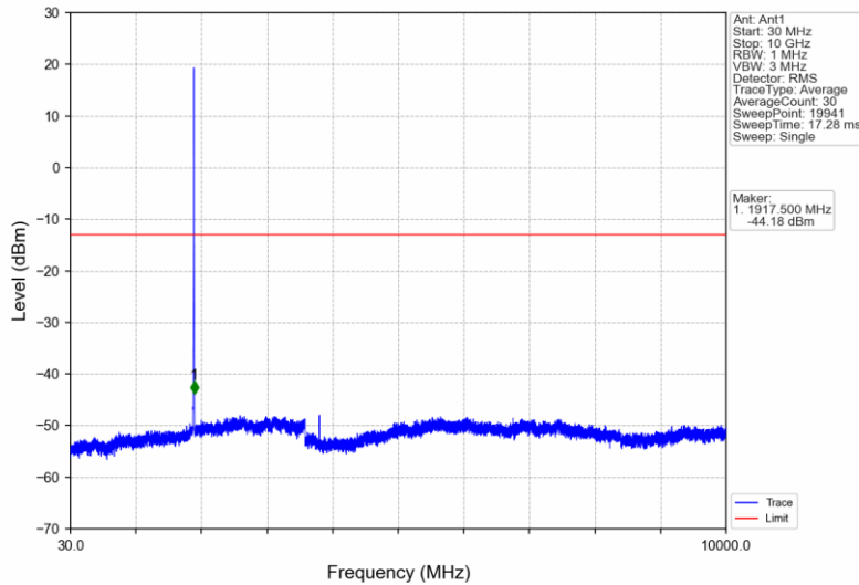
BandII_RMC_HCH_1907.6MHz_12.2kbps RMC_NTNV
