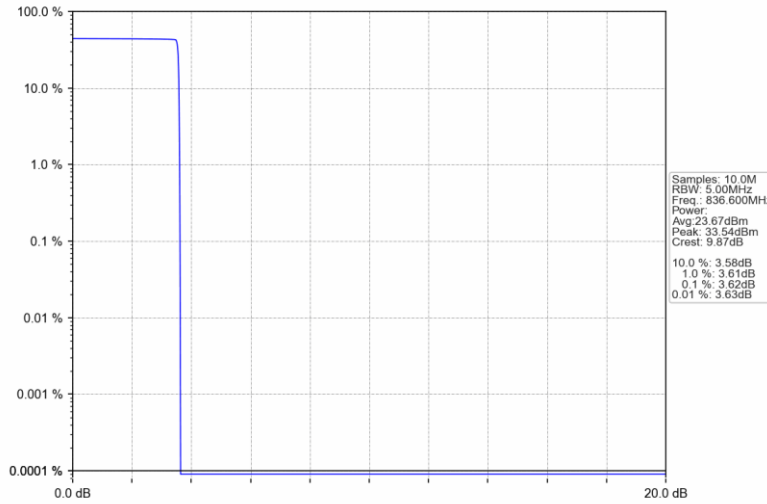
GSM850_GPRS_MCH_836.6MHz_4 TX Slots_NTNV
