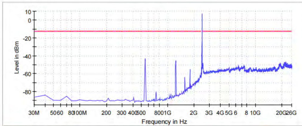
Spurious
