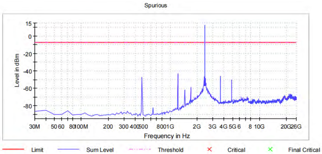
DH5_Ant1_2441_30~26500
