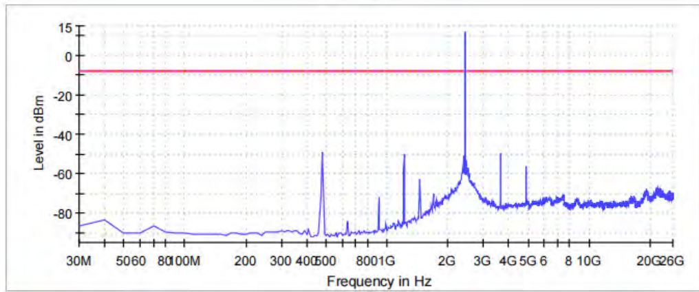
Spurious
