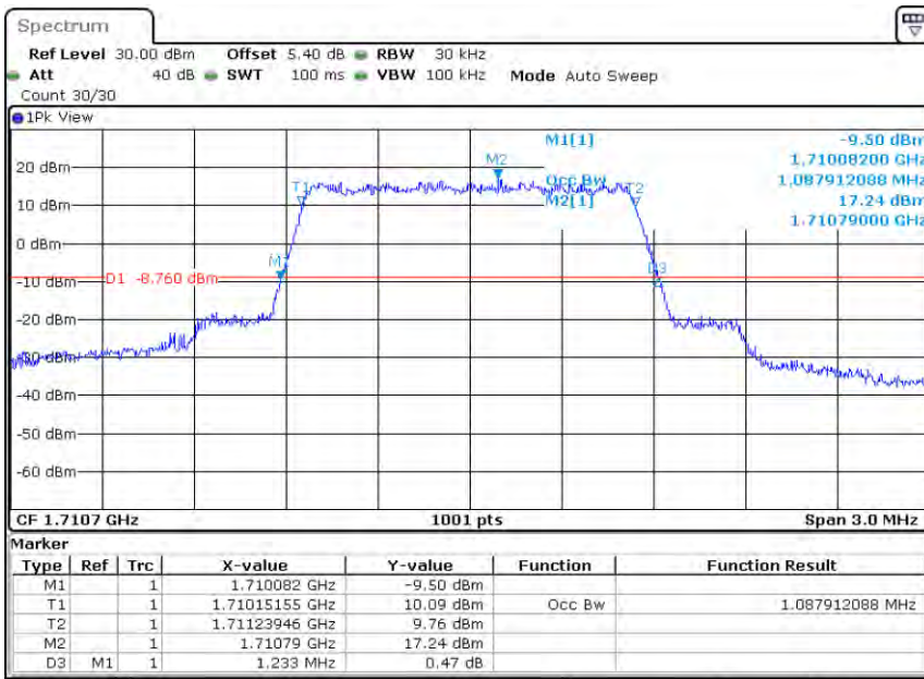
Band66-1.4MHz-QPSK-131979-6RB#0-1.088
