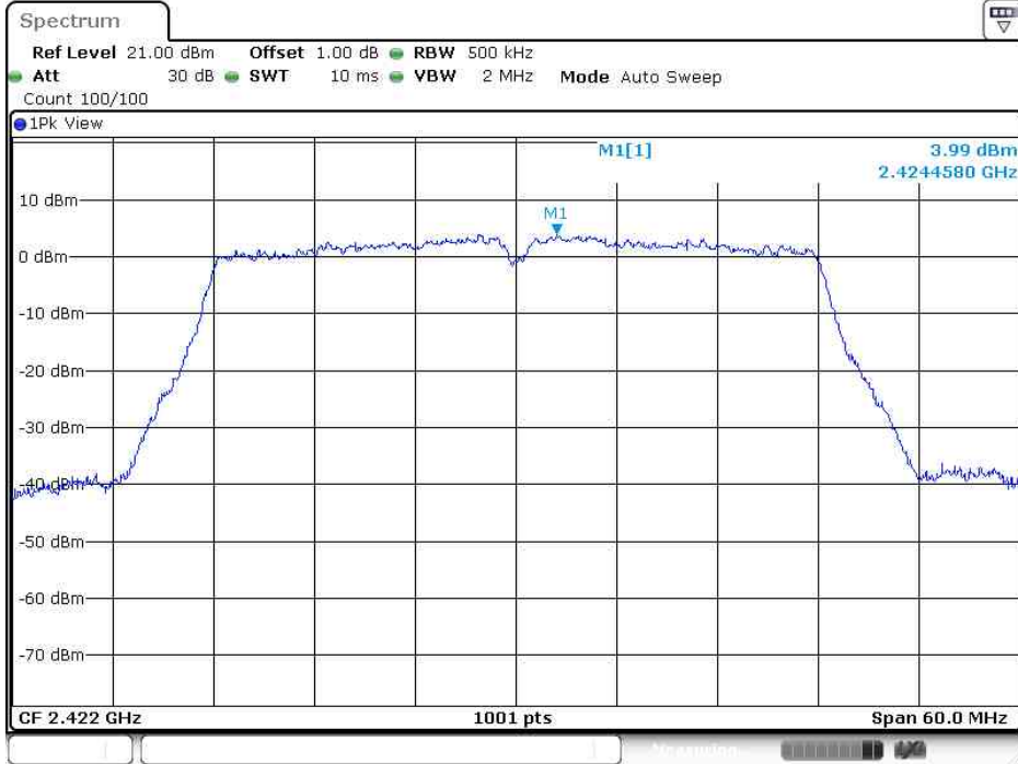
11N40SISO_Ant1_2422
