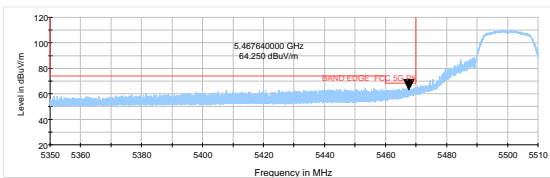
802.11a-Channel 100: Peak
