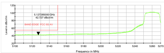
802.11a-Channel 52: Average
