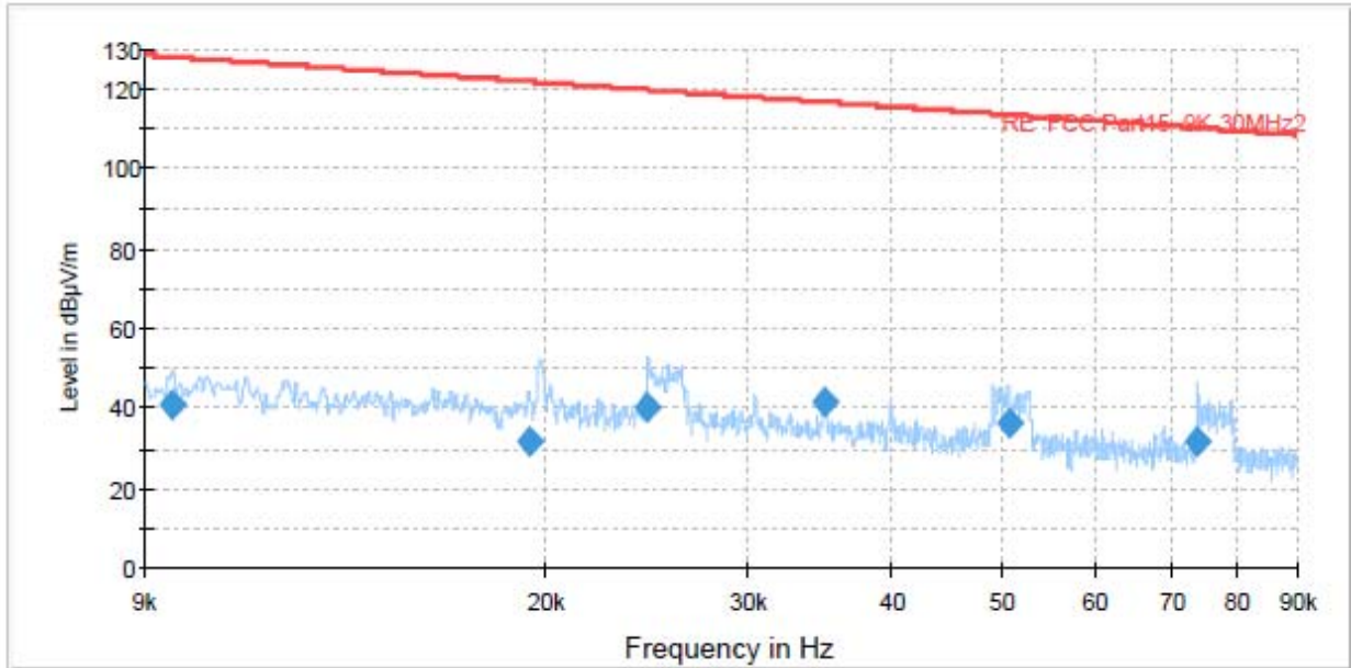
Radiates Emission from 9kHz to 90kHz
