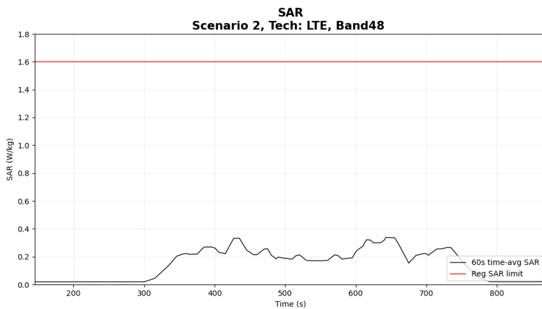
Figure 6- 24 Time-averaged SAR
