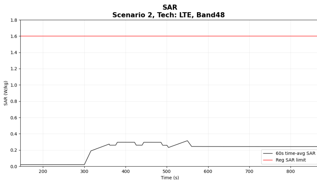
Figure 6- 22 Time-averaged SAR
