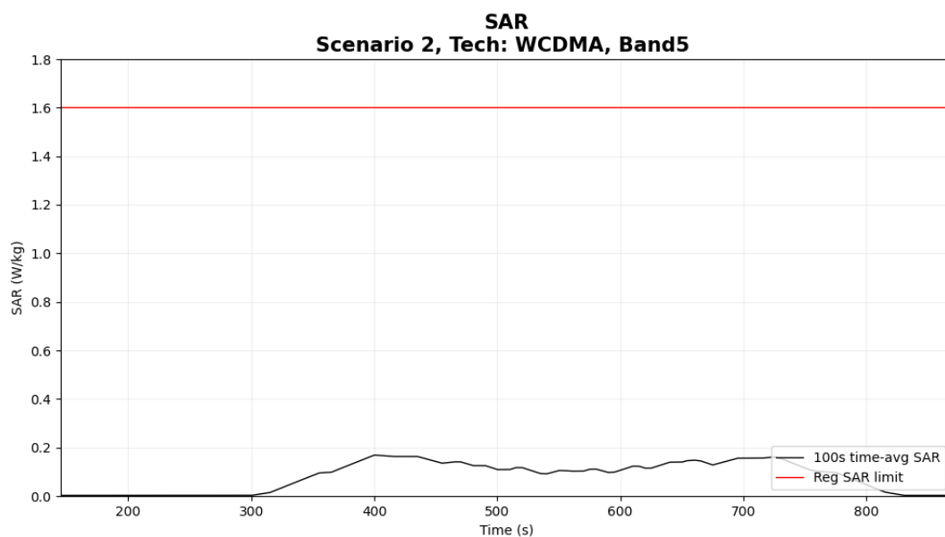
Figure 6- 17 Time-averaged SAR
