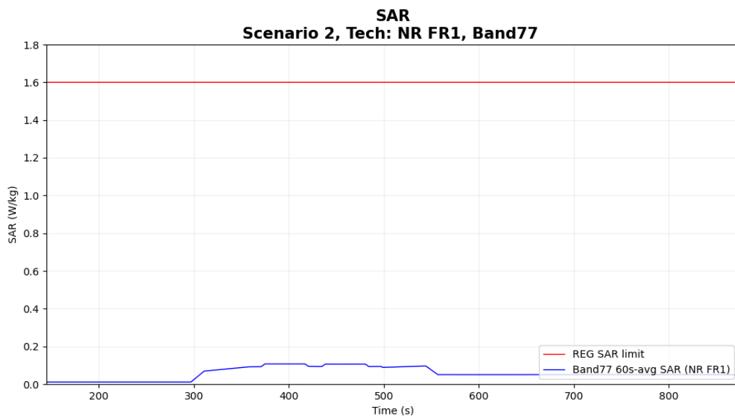
Figure 7-5 Time-averaged SAR
