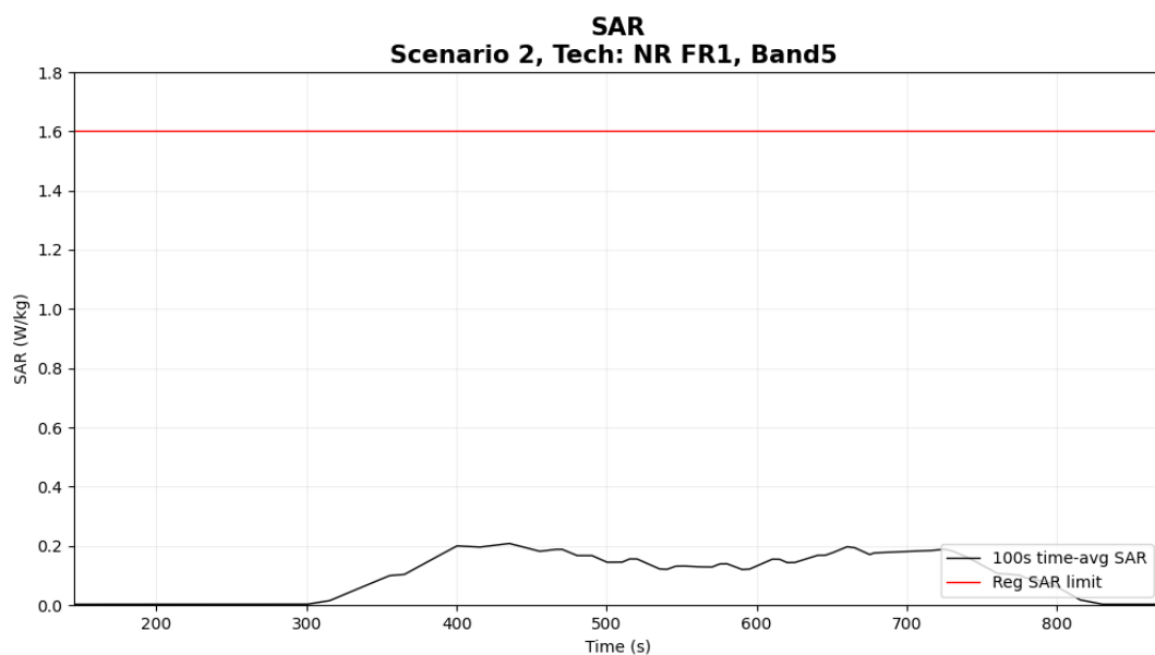
Figure 6- 28 Time-averaged SAR
