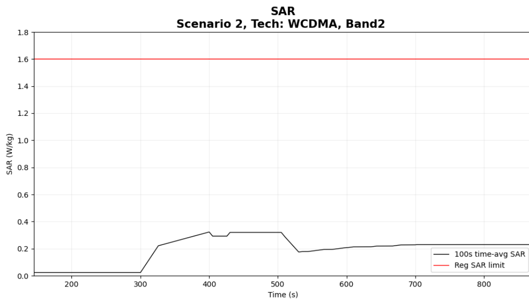
figure 6- 12 Time-averaged SAR
