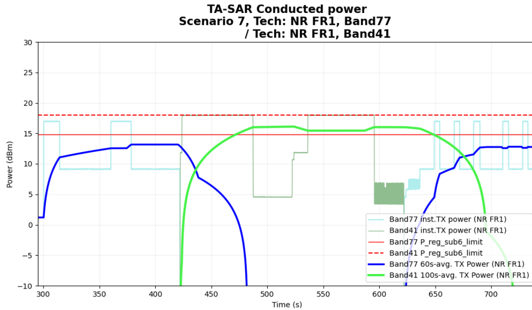
Figure 6- 38 Time-averaged conducted TX power over time
