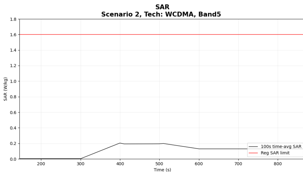
Figure 6- 15 Time-averaged SAR
