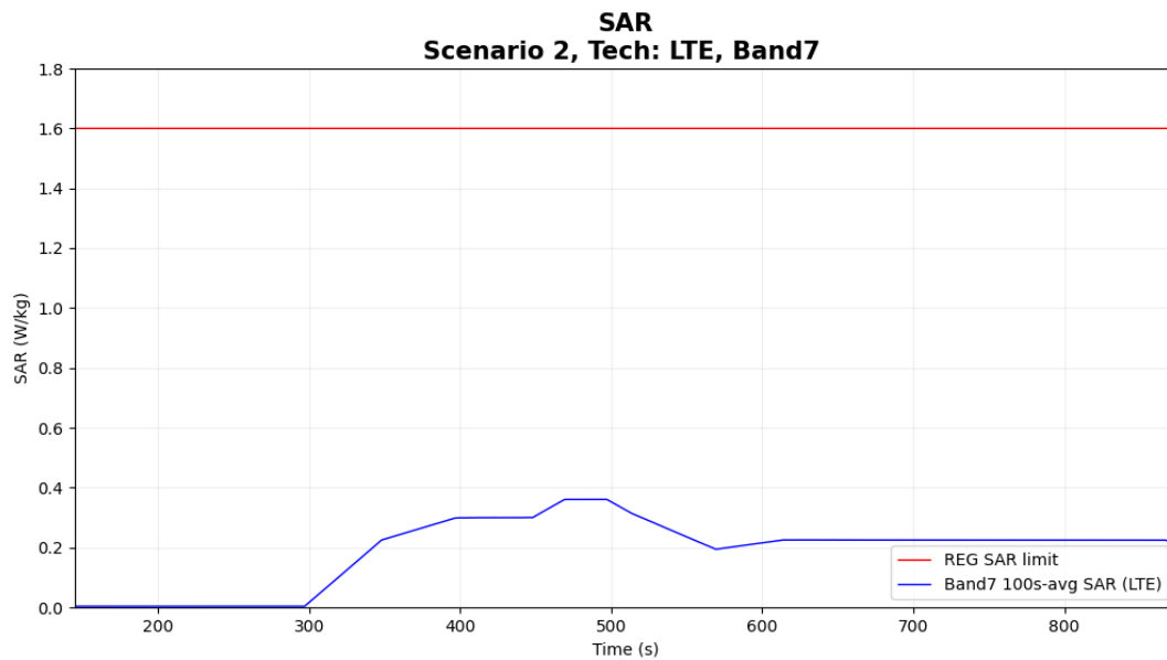
Figure 7-7 Time-averaged SAR
