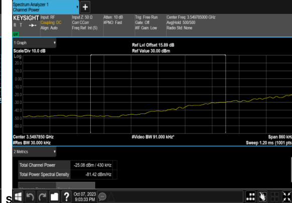
N48(40M)_DFT-s- OFDM_BPSK_Edge_1RB_Left_Low_CH_CHP_PAS
