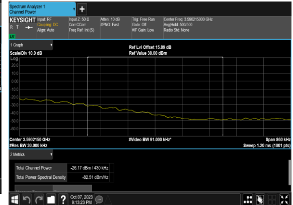
N48(40M)_DFT-s- OFDM_BPSK_Edge_1RB_Right_Low_CH_CHP_P ASS
