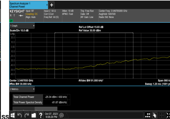
N48(40M)_DFT-s- OFDM_QPSK_Edge_1RB_Left_Low_CH_CHP_PA
