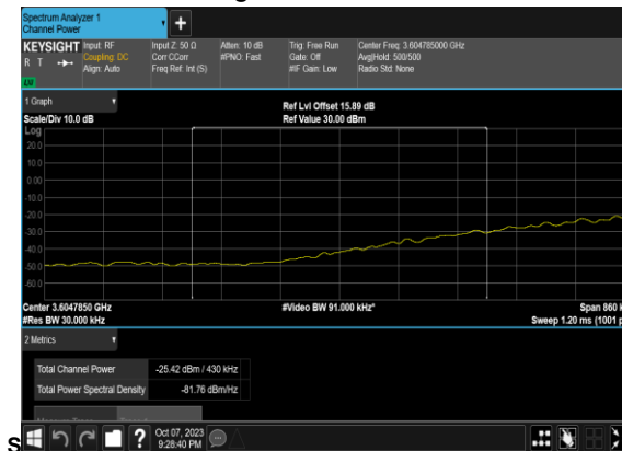
N48(40M)_DFT-s- OFDM_BPSK_Edge_1RB_Left_Mid_CH_CHP_PAS
