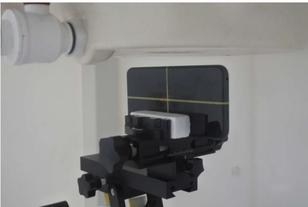
Left Side, Test Separation 15 mm(sensor off)
