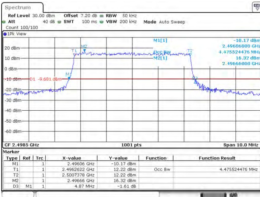
Band41-5MHz-QPSK-39675-25RB#0-4.476
