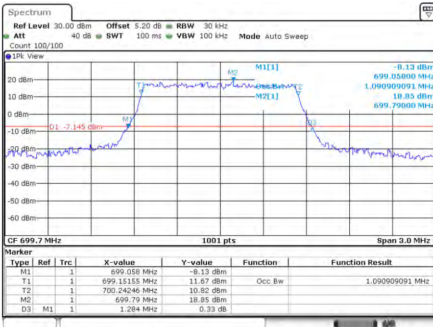
Band12-1.4MHz-QPSK-23017-6RB#0-1.091
