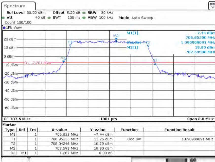
Band12-1.4MHz-QPSK-23095-6RB#0-1.091
