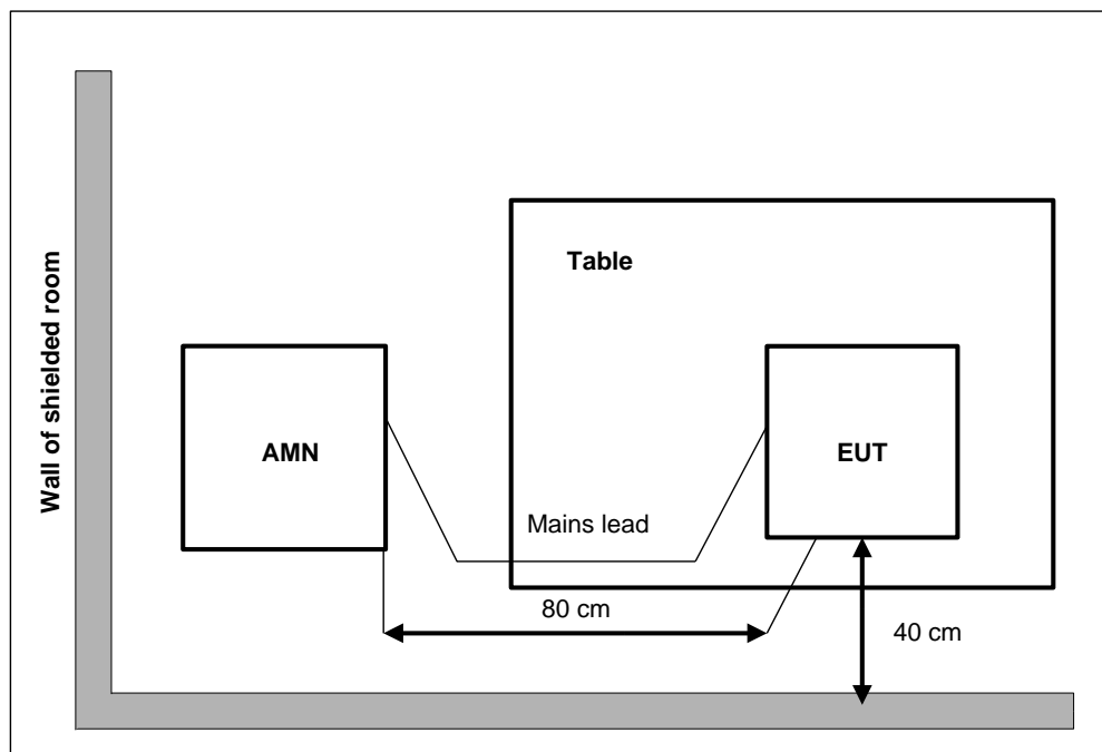
Figure A-8: Measurement Setup
