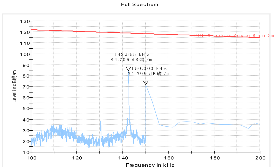
Figure A-2: Traffic Mode(distance = 3m, Using wireless charger)
