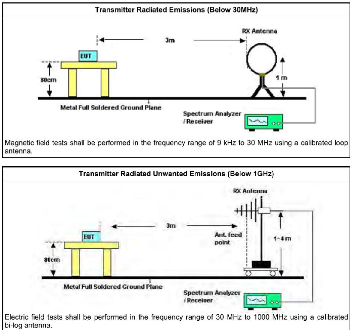
Figure A-1: Measurement Setup
