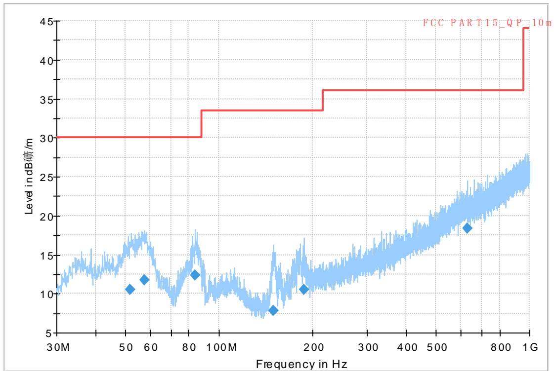
Figure A-7: Traffic Mode(distance = 10m, Using Phone, 30MHz-1GHz)
