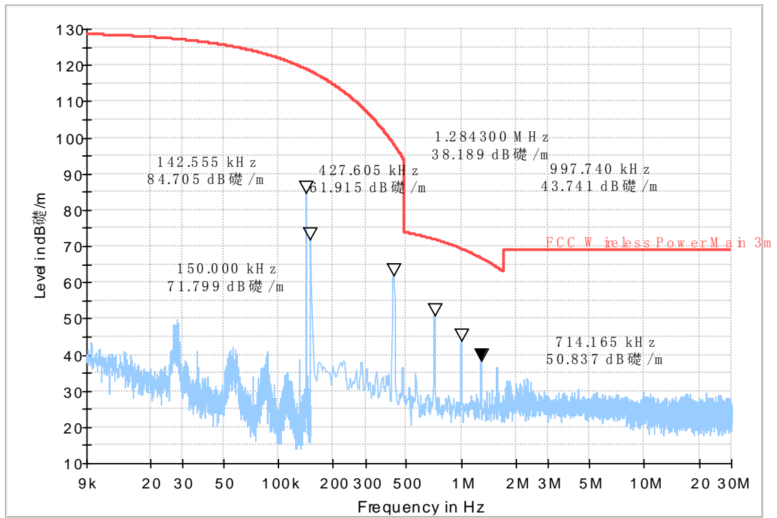
Figure A-3: Traffic Mode(distance = 3m, Using wireless charger, 9kHz-30MHz)
