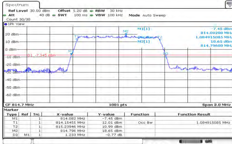
Band26-1.4MHz-QPSK-26697-6RB#0-1.085
