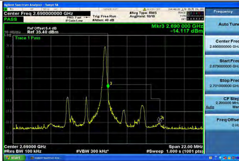
Band41-5MHz-64QAM-41565-25RB#0
