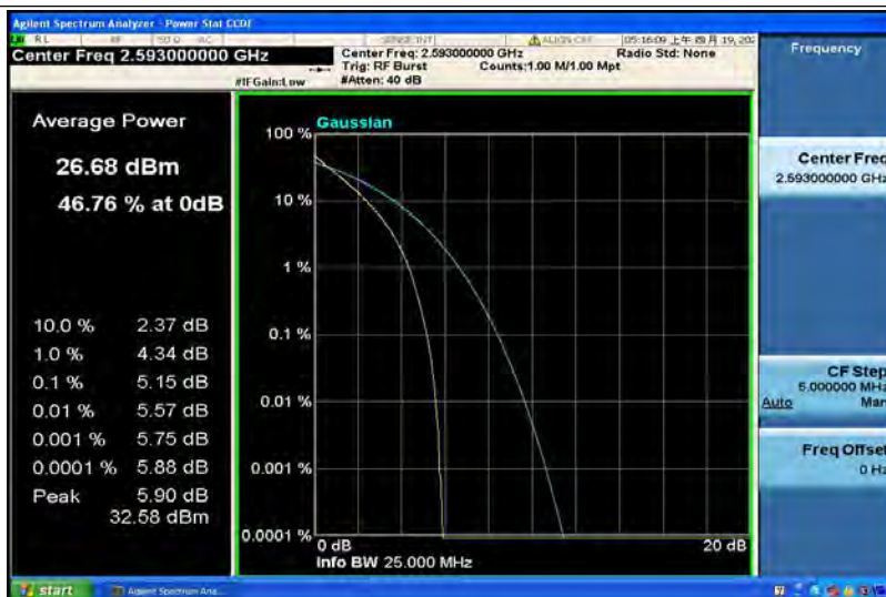
Band41-20MHz-QPSK-41490-100RB#0
