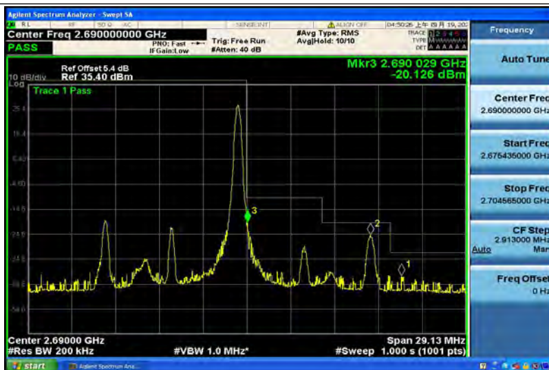
Band41-10MHz-QPSK-41540-50RB#0
