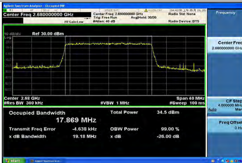
Band41-20MHz-16QAM-41490-100RB#0-17.869
