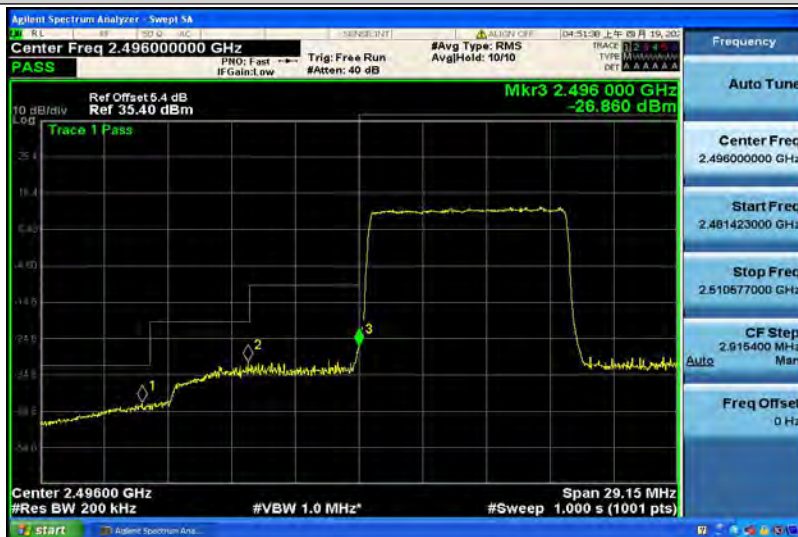
Band41-10MHz-QPSK-41540-1RB#49
