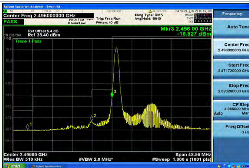
Band41-20MHz-64QAM-39750-100RB#0
