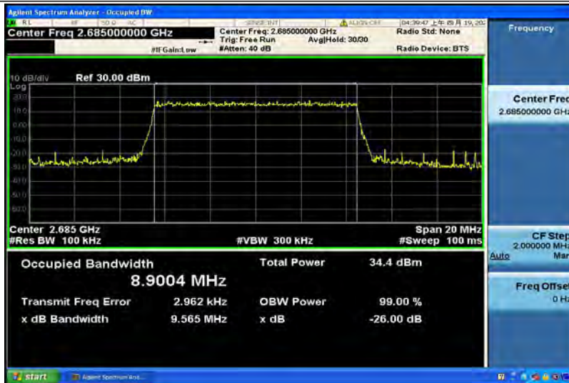
Band41-10MHz-64QAM-39700-50RB#0-8.9117
