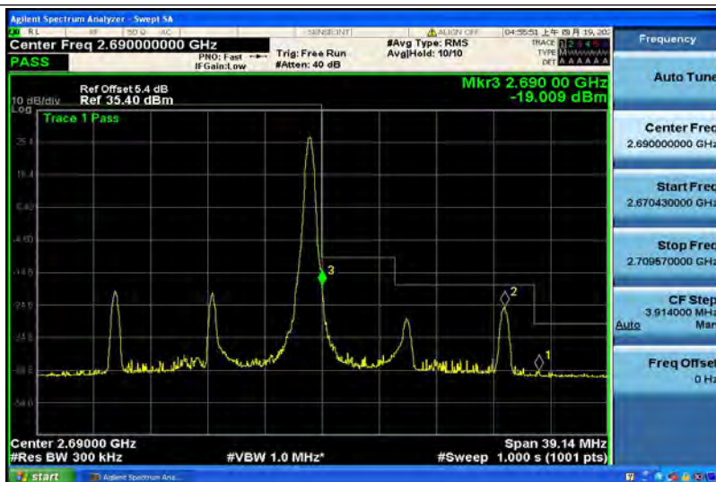
Band41-15MHz-64QAM-41515-75RB#0
