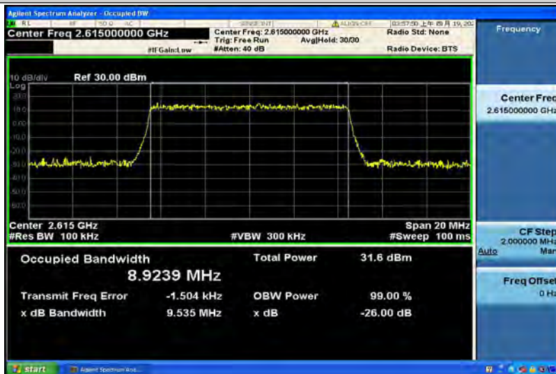
Band38-15MHz-QPSK-37825-75RB#0-13.460
