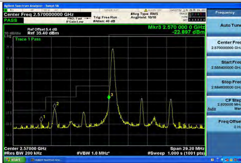
Band38-10MHz-64QAM-37800-50RB#0
