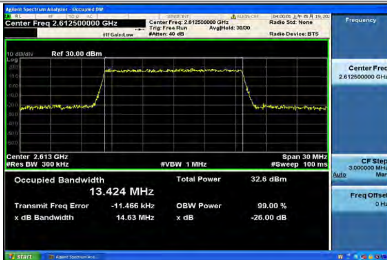
Band38-15MHz-16QAM-37825-75RB#0-13.442
