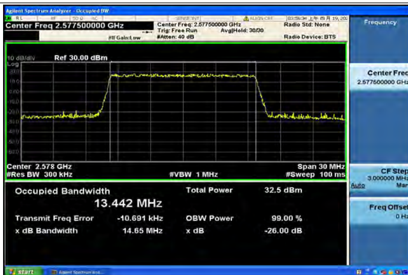
Band38-15MHz-16QAM-38000-75RB#0-13.422
