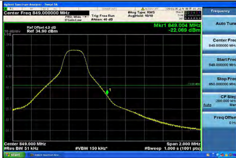
Band5-5MHz-64QAM-20625-25RB#0
