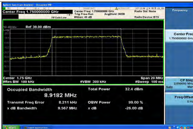
Band4-10MHz-16QAM-20000-50RB#0-8.9255
