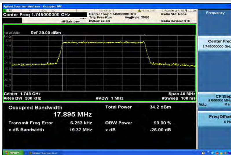
Band4-20MHz-64QAM-20050-100RB#0-17.868
