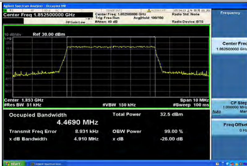
Band2-5MHz-64QAM-18900-25RB#0-4.4679
