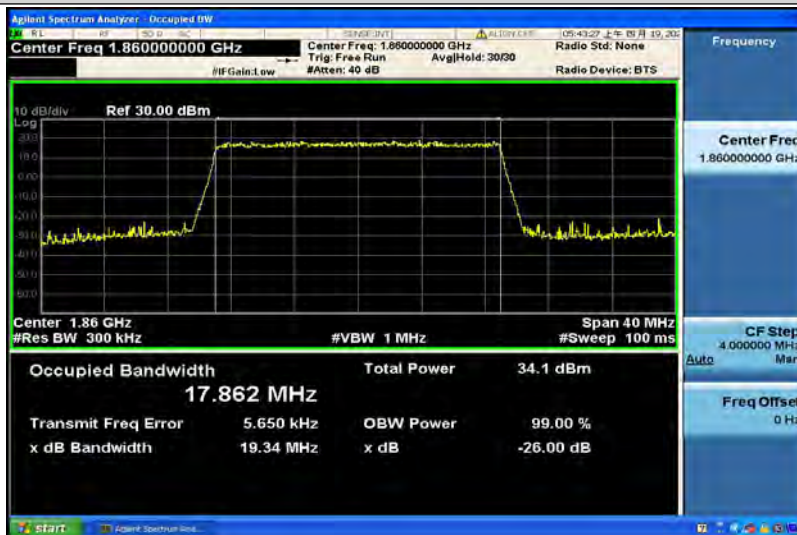
Band2-20MHz-QPSK-18900-100RB#0-17.869
