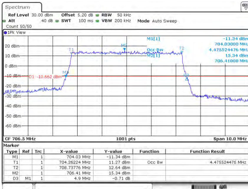
Band17-5MHz-QPSK-23755-25RB#0-4.476
