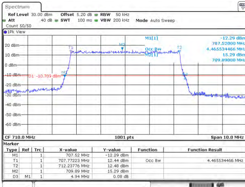
Band17-5MHz-QPSK-23790-25RB#0-4.466
