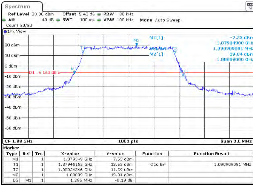
Band2-1.4MHz-QPSK-18900-6RB#0-1.091
