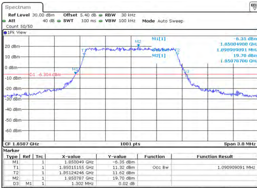
Band2-1.4MHz-QPSK-18607-6RB#0-1.091
