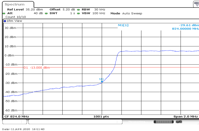
Band5-1.4MHz-64QAM-20643-1RB#5
