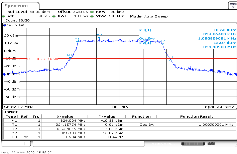
Band5-1.4MHz-64QAM-20525-6RB#0-1.091
