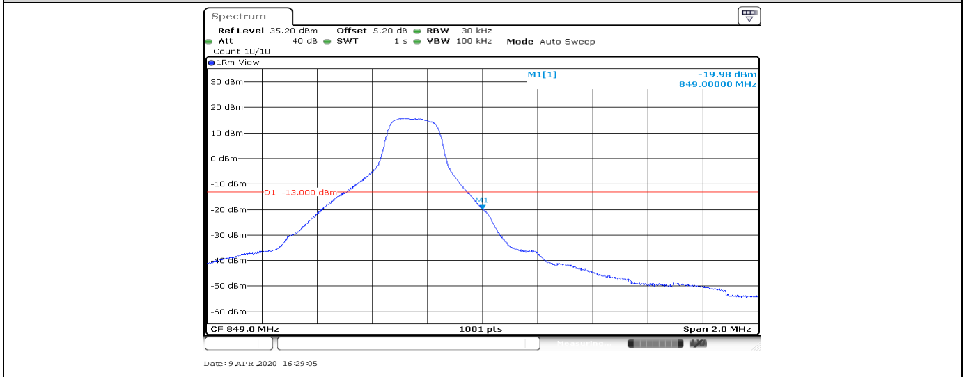
Band5-1.4MHz-QPSK-20643-6RB#0
