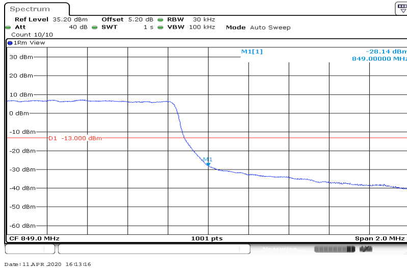
Band5-1.4MHz-64QAM-20407-1RB#0
