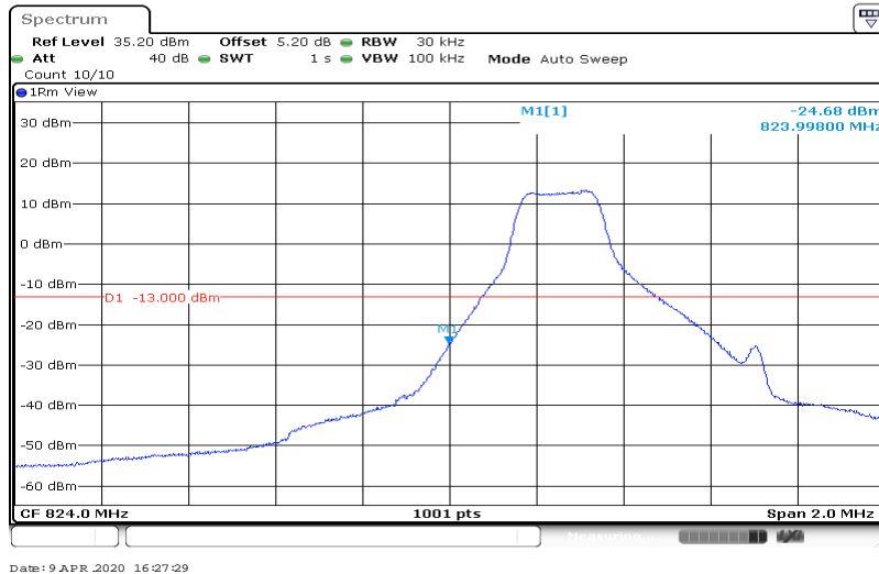
Band5-1.4MHz-64QAM-20407-6RB#0
