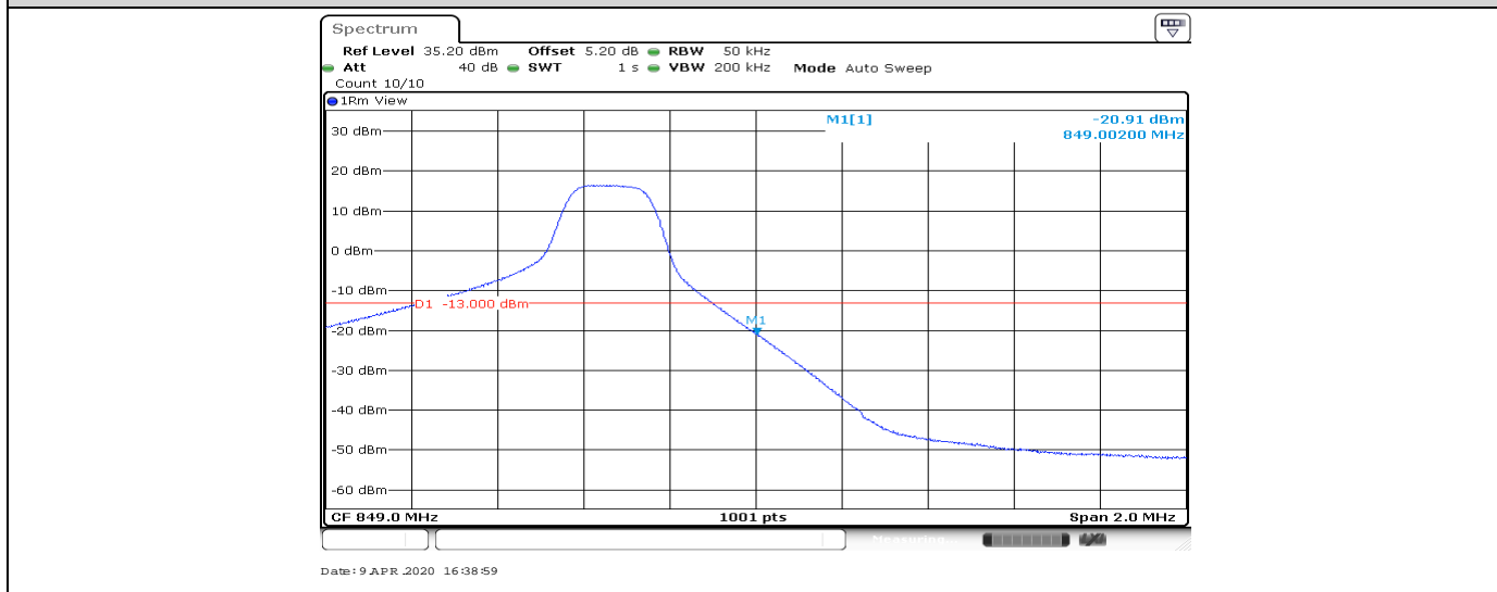
Band5-5MHz-16QAM-20625-25RB#0
