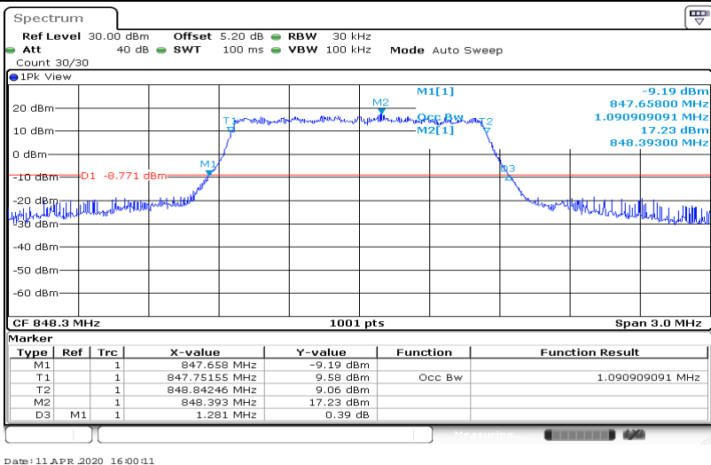
Band5-1.4MHz-64QAM-20407-6RB#0-1.091
