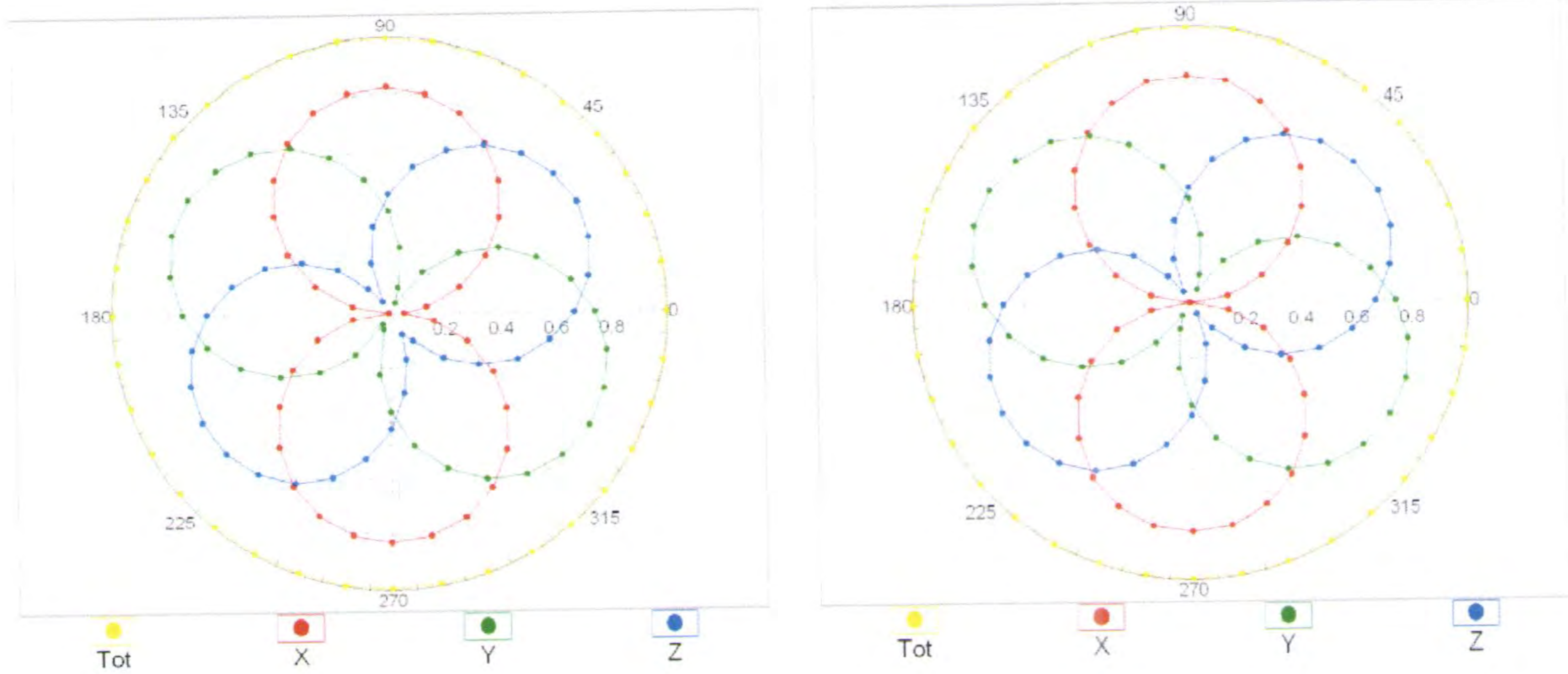
f=600 MHz,TEM
