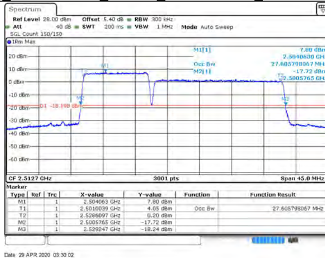
CA 7C 50RB+100RB 64QAM 21006+21150 50RB#0+100RB#0
