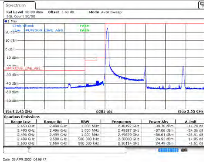
CA 7C 100RB+100RB 64QAM 20850+21048 100RB#0+100RB#0
