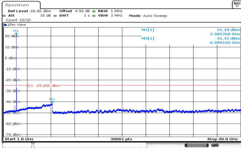
Band38-20MHz-16QAM-38000-1RB#0-Range2:1000~30000MHz
