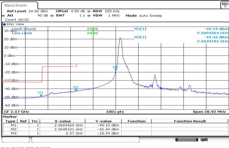
Band38-10MHz-16QAM-37800-50RB#0
