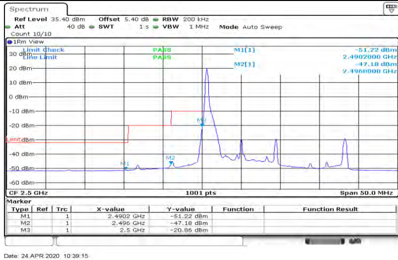
Band7-10MHz-64QAM-20800-50RB#0
