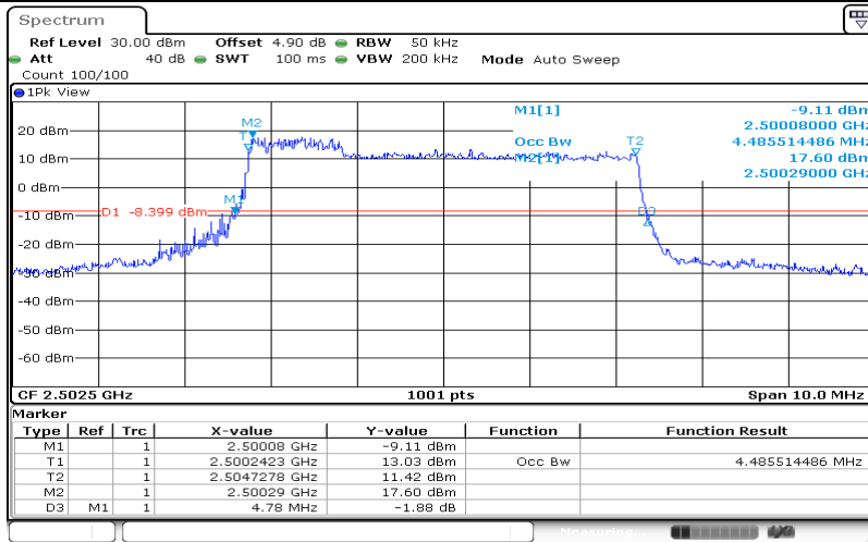
Band7-5MHz-QPSK-20775-25RB#0-4.486
