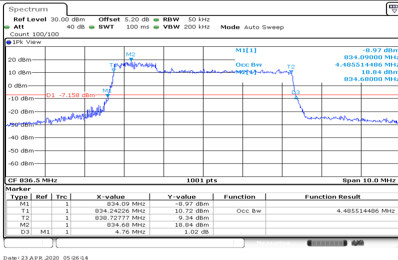
Band5-5MHz-16QAM-20625-25RB#0-4.486
