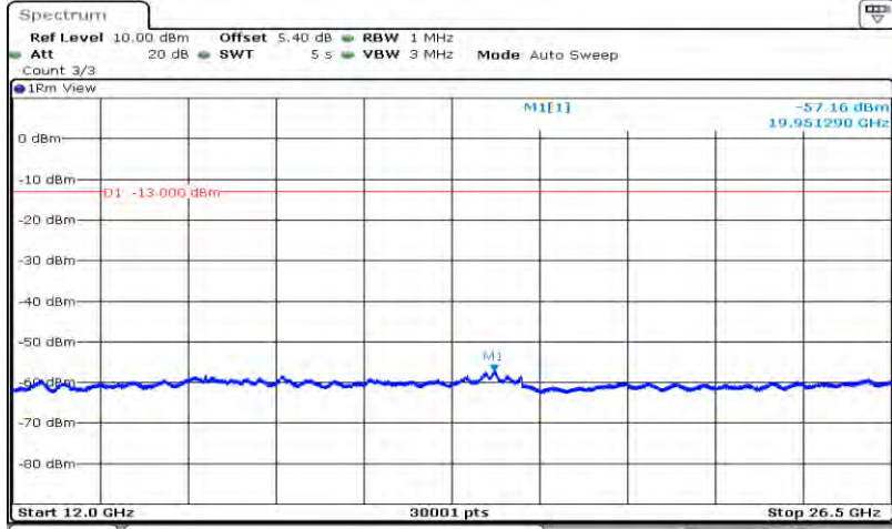
Band5-10MHz-64QAM-20525-1RB#0-Range4:12000~26500MHz
