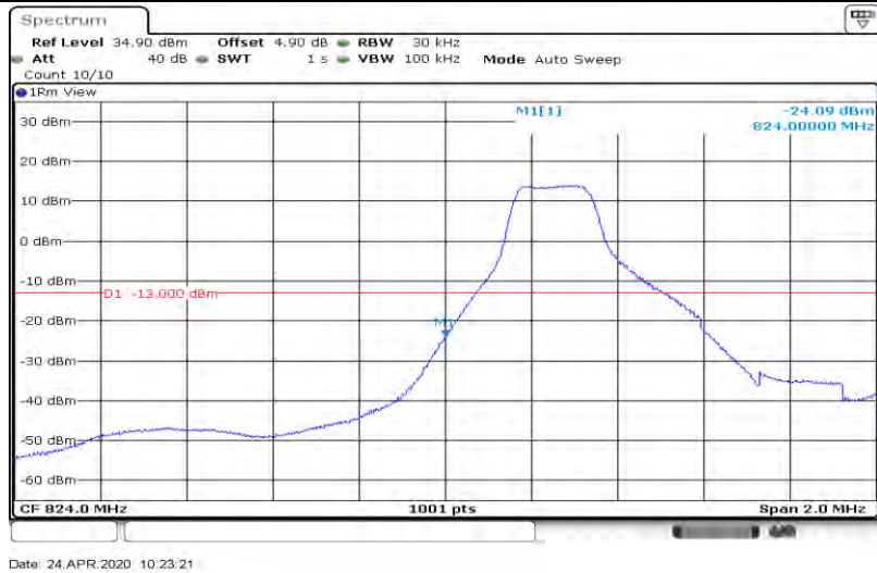
Band5-1.4MHz-64QAM-20407-6RB#0
