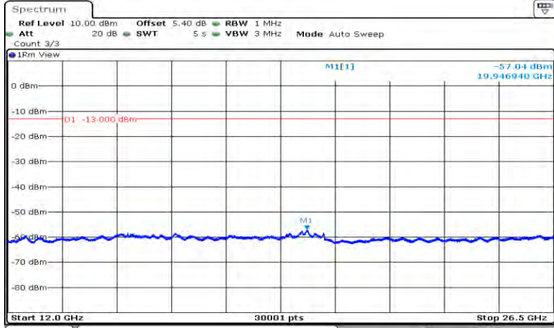
Band5-10MHz-64QAM-20450-1RB#0-Range4:12000~26500MHz
