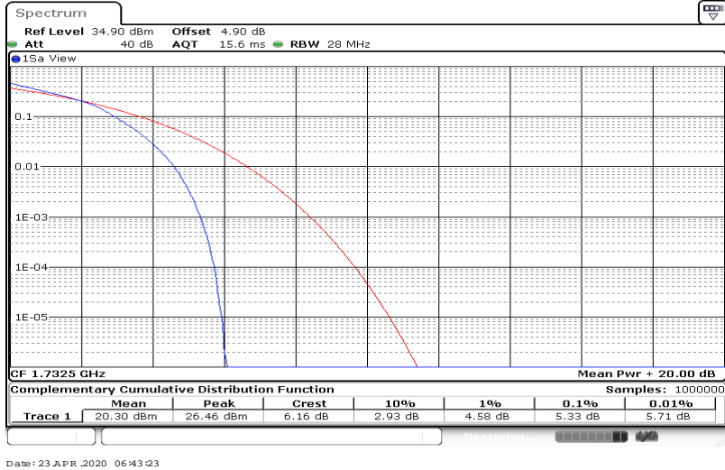
Band4-20MHz-64QAM-20300-100RB#0
