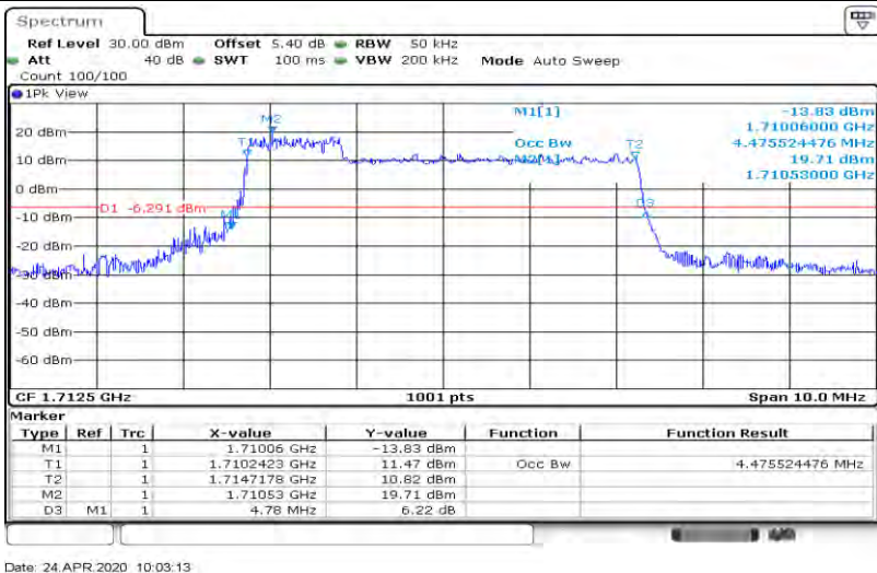
Band4-5MHz-64QAM-20175-25RB#0-4.476
