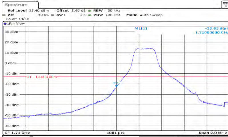
Band4-1.4MHz-64QAM-19957-6RB#0
