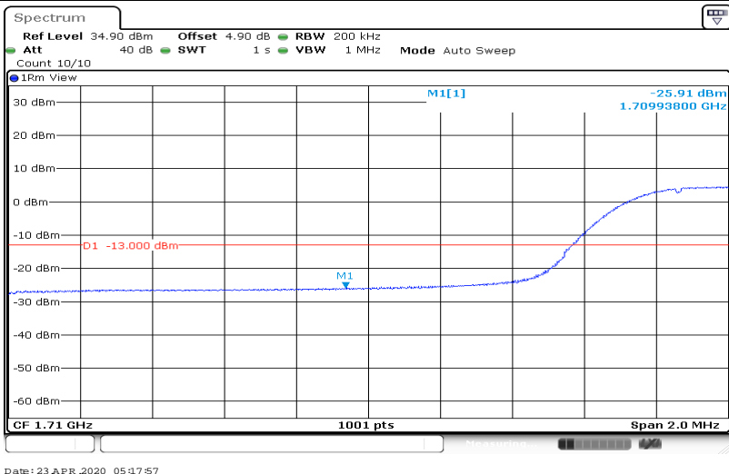
Band4-15MHz-QPSK-20325-1RB#74
