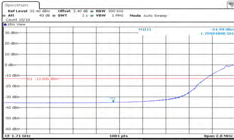
Band4-20MHz-64QAM-20050-100RB#0
