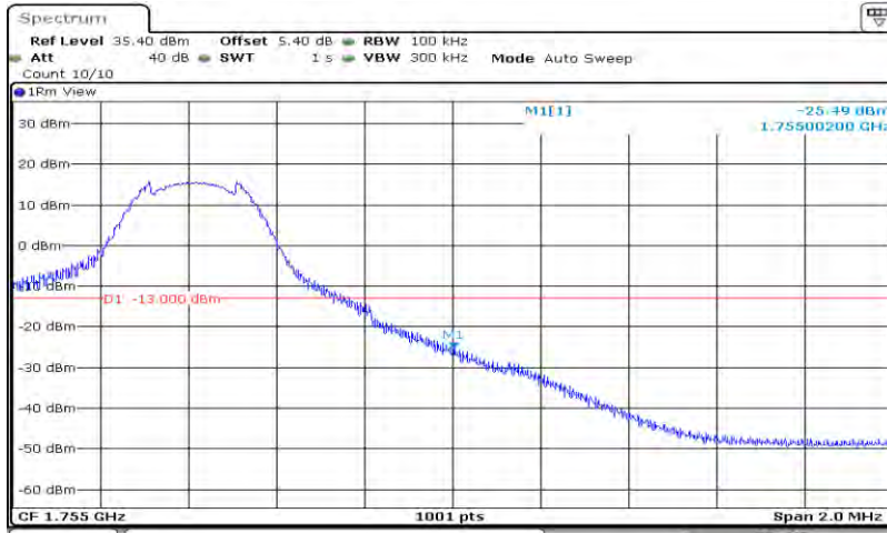
Band4-10MHz-64QAM-20350-50RB#0
