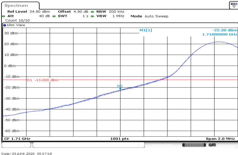
Band4-15MHz-QPSK-20025-75RB#0
