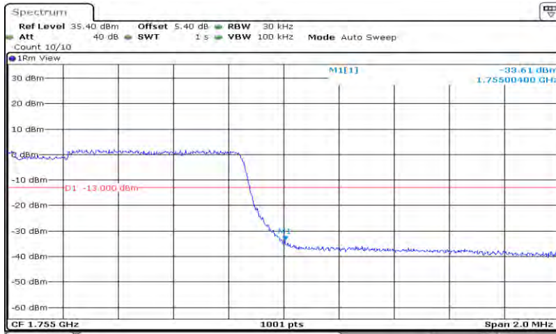
Band4-3MHz-64QAM-20385-15RB#0
