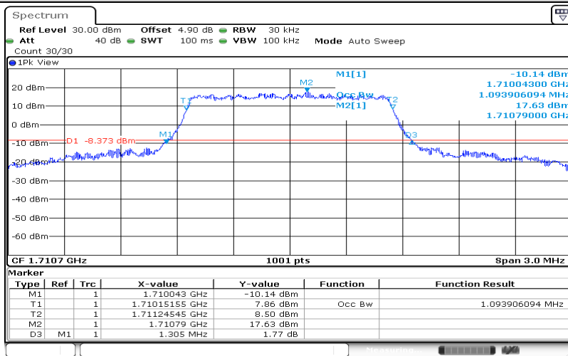
Band4-1.4MHz-QPSK-19957-6RB#0-1.094
