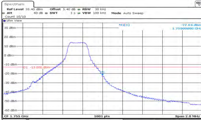
Band4-1.4MHz-64QAM-20393-6RB#0
