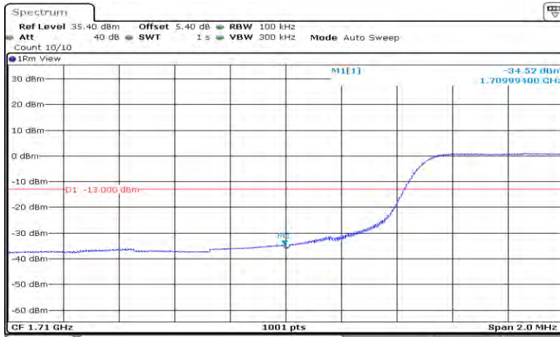
Band4-10MHz-64QAM-20000-50RB#0
