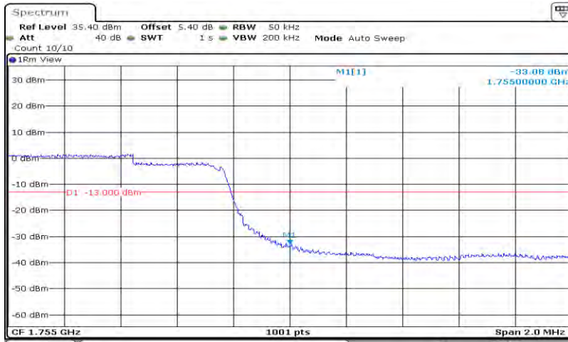
Band4-5MHz-64QAM-20375-25RB#0
