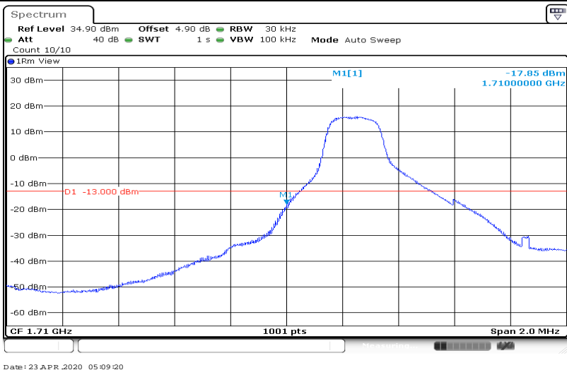
Band4-3MHz-QPSK-19965-15RB#0
