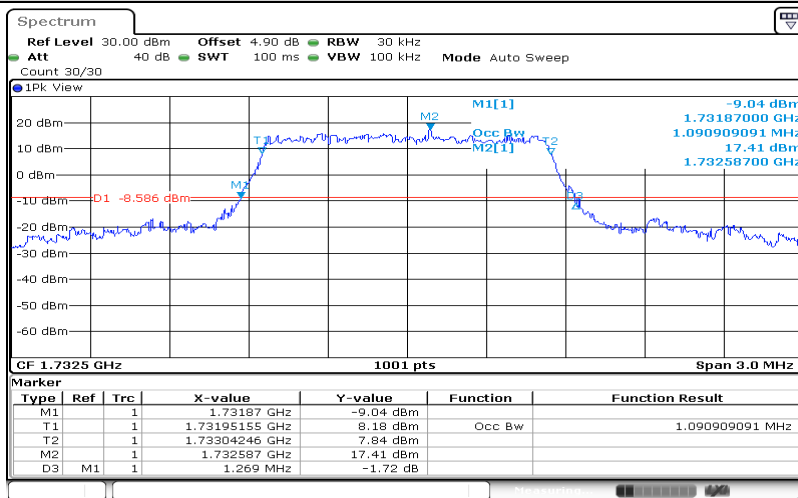
Band4-1.4MHz-QPSK-20175-6RB#0-1.091
