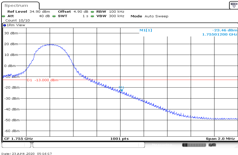
Band4-10MHz-16QAM-20350-50RB#0
