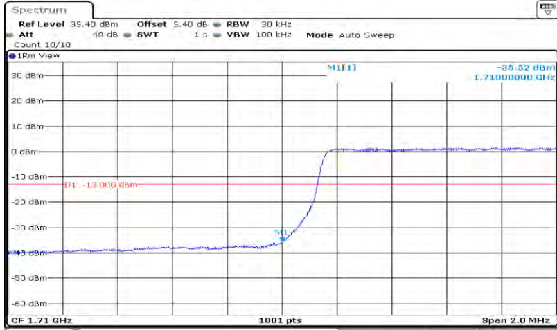
Band4-3MHz-64QAM-19965-15RB#0
