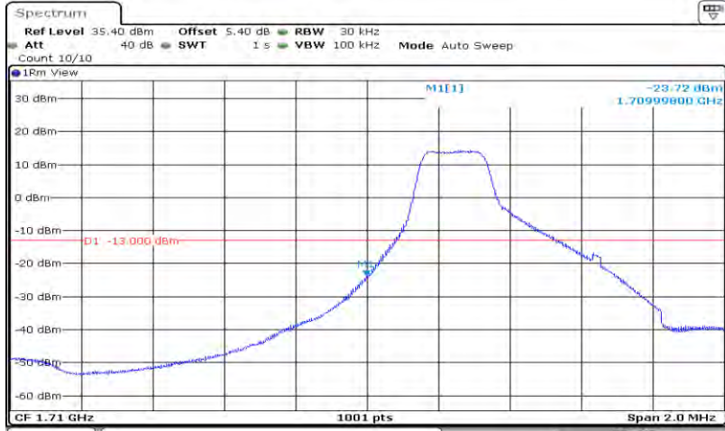
Band4-3MHz-64QAM-19965-15RB#0
