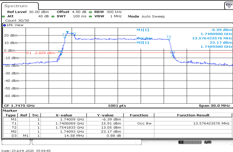
Band4-15MHz-64QAM-20025-75RB#0-13.576
