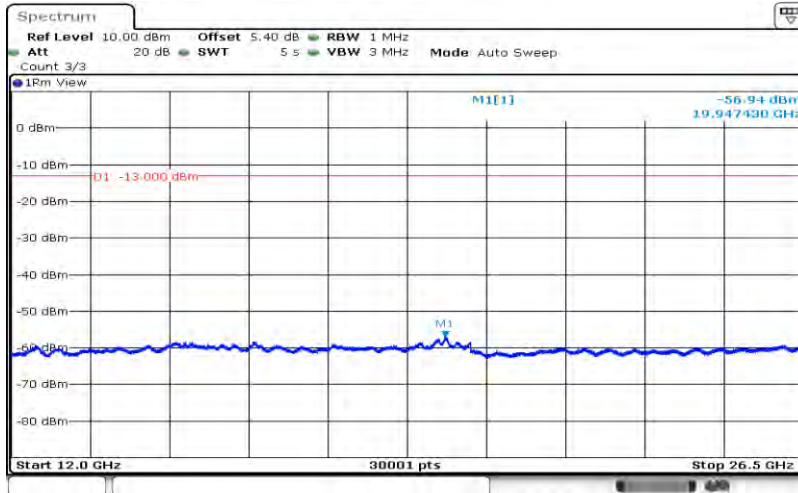
Band2-20MHz-64QAM-19100-1RB#0-Range4:12000~26500MHz
