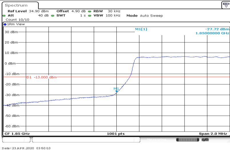
Band2-1.4MHz-16QAM-19193-1RB#5
