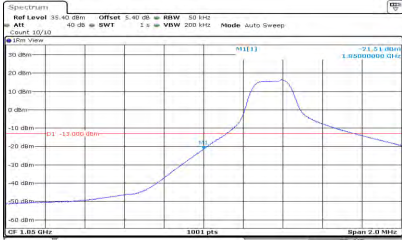
Band2-5MHz-64QAM-18625-25RB#0
