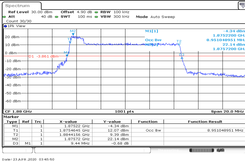
Band2-10MHz-16QAM-19150-50RB#0-8.951
