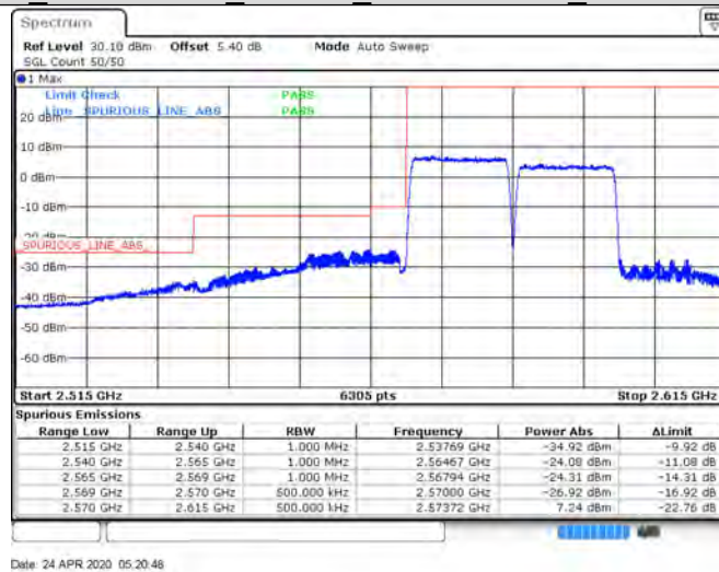
CA 38C 75RB+75RB 64QAM 38025+38175 0RB#0+1RB#74
