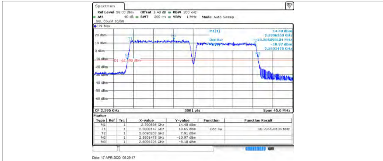
CA 38C 15MHz+15MHz 16QAM 38025+38175 75RB#0+75RB#0
