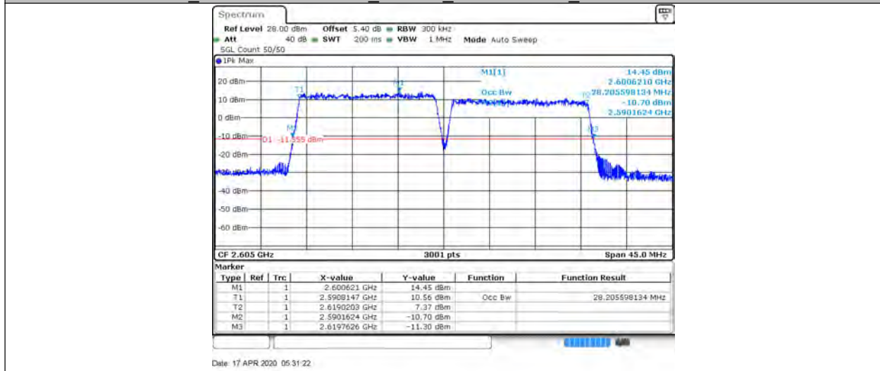
CA 38C 15MHz+15MHz 64QAM 37825+37975 75RB#0+75RB#0
