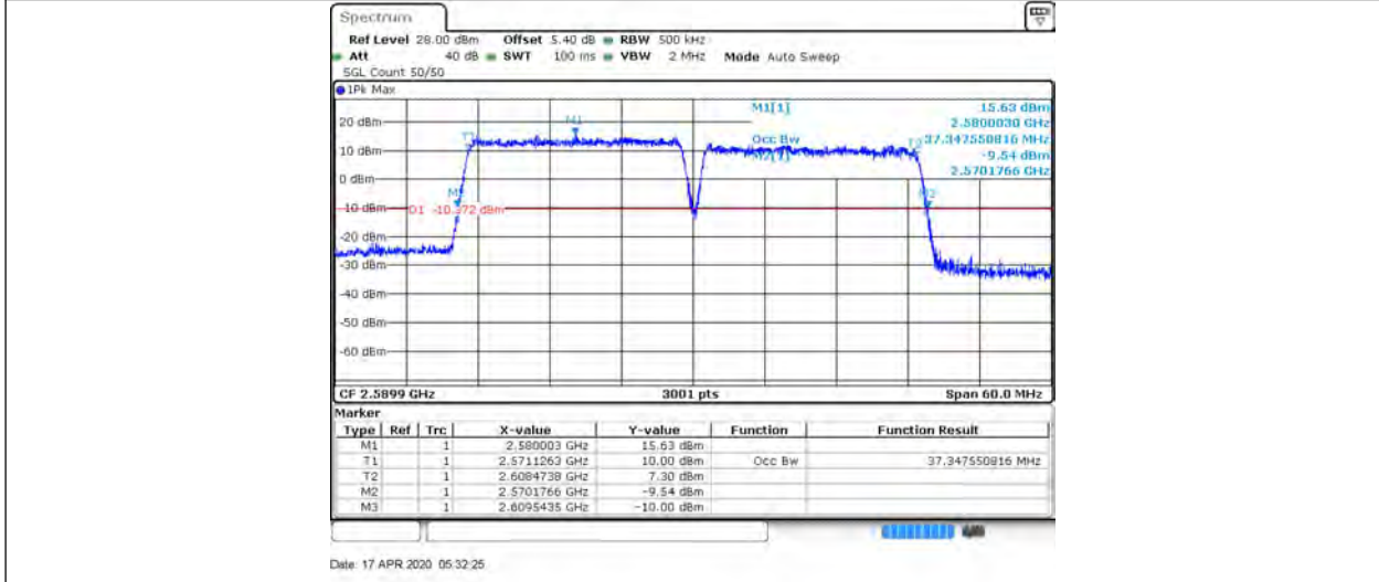
CA_38C_20MHz+20MHz_64QAM_37901+38099_100RB#0+100RB#0
