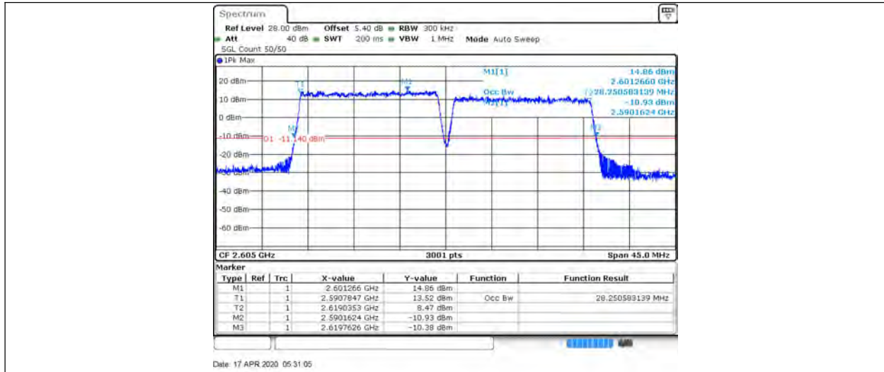
CA 38C 15MHz+15MHz 16QAM 37825+37975 75RB#0+75RB#0
