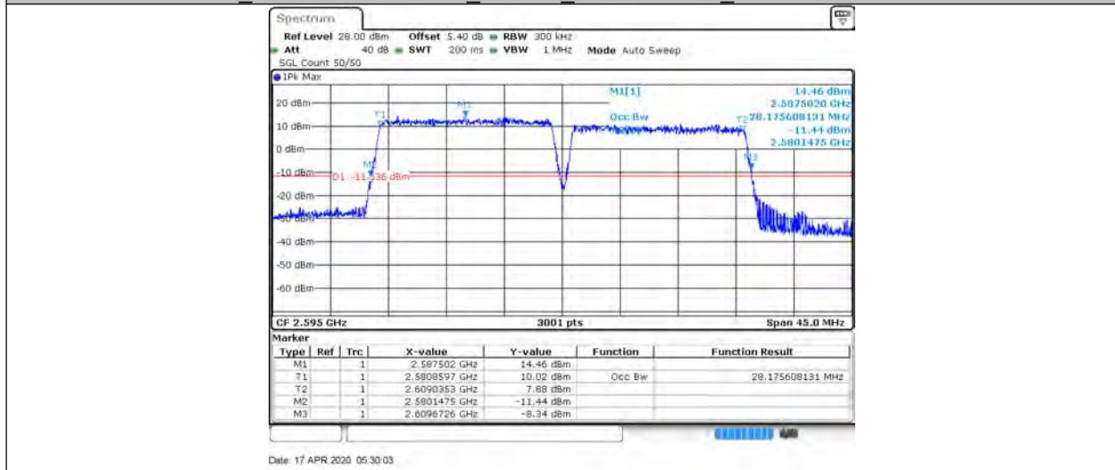
CA_38C_15MHz+15MHz_64QAM_38025+38175_75RB#0+75RB#0
