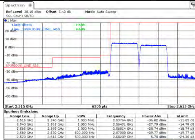
CA_38C_75RB+75RB_QPSK_37825+37975_75RB#0+75RB#0
