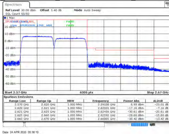
CA_38C_100RB+100RB_16QAM_37850+38048_1RB#0+0RB#0
