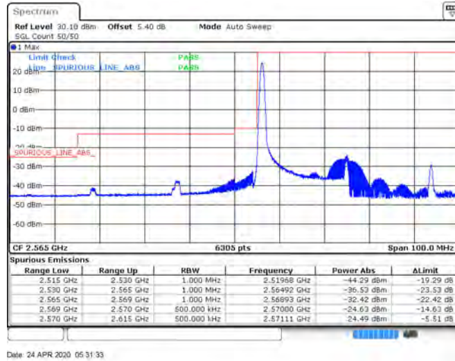
CA_38C_100RB+100RB_QPSK_37850+38048_100RB#0+100RB#0
