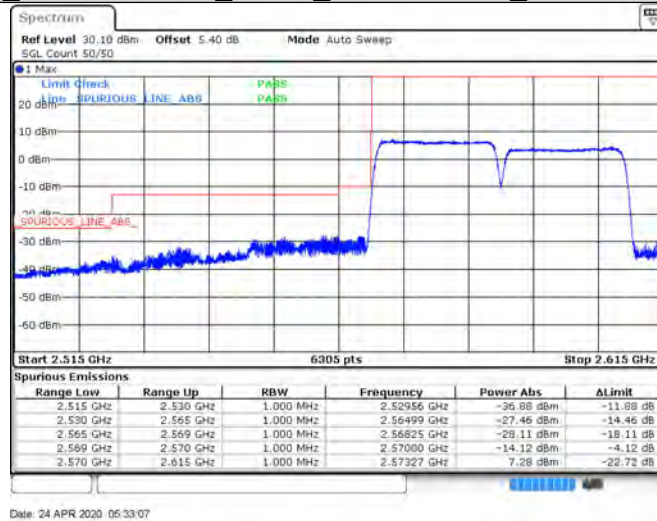
CA_38C_100RB+100RB_QPSK_37952+38150_0RB#0+1RB#99
