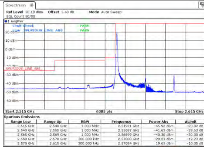
CA_38C_75RB+75RB_QPSK_37825+37975_1RB#0+0RB#0
