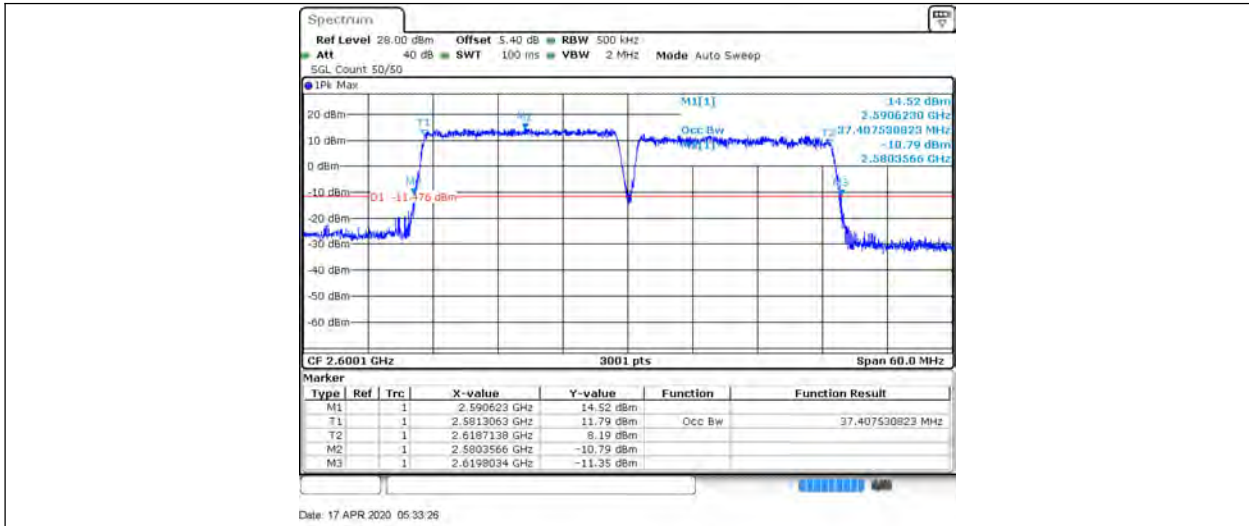
CA_38C_20MHz+20MHz_64QAM_37850+38048_100RB#0+100RB#0
