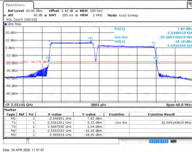
CA_7C_15+20_64QAM_20828+20999_75RB#0+100RB#0
