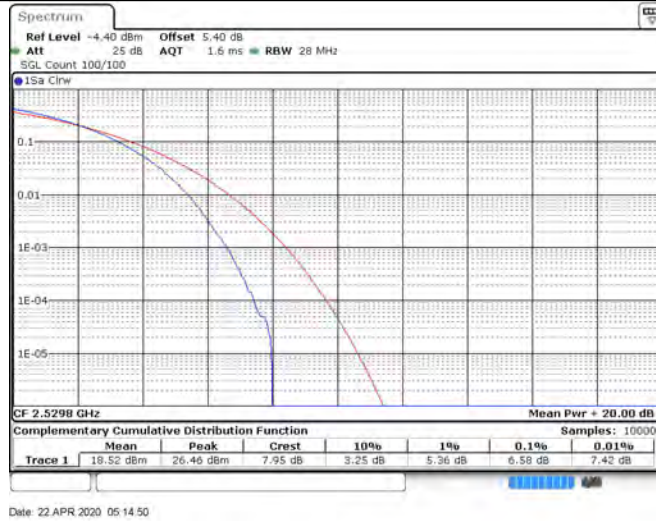
CA 7C 100RB+100RB 16QAM 2119+21001 100RB#0+100RB#0
