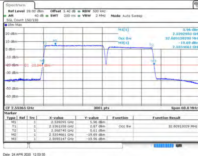
CA_7C_20+15_64QAM_20850+21021_100RB#0+75RB#0
