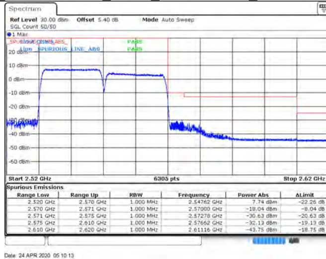
CA_7C_100RB+100RB_16QAM_20850+21048_1RB#0+0RB#0
