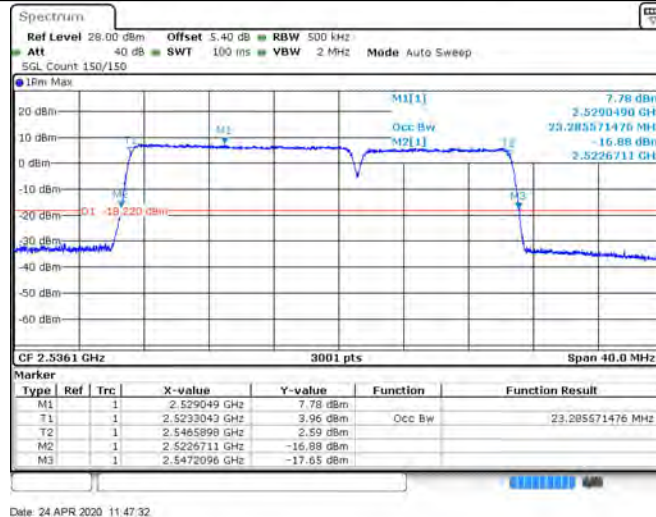
CA_7C_15+10_64QAM_21277+21397_75RB#0+50RB#0
