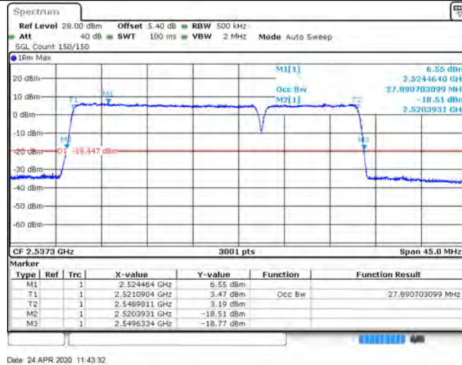
CA_7C_20+10_16QAM_21251+21395_100RB#0+50RB#0
