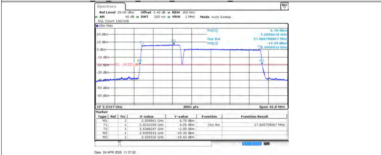
CA_7C_10+20_16QAM_21006+21150_50RB#0+100RB#0
