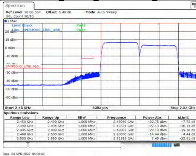
CA 7C 100RB+100RB 16QAM 21152+21350 0RB#0+1RB#99
