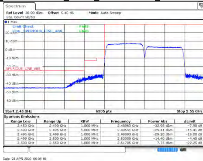
CA_7C_100RB+100RB_QPSK_21152+21350_0RB#0+1RB#99
