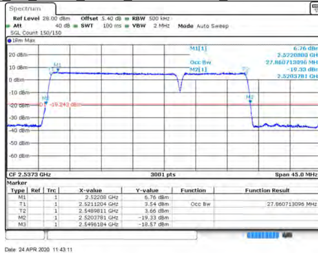
CA 7C_20+10_QPSK_21251+21395_100RB#0+50RB#0
