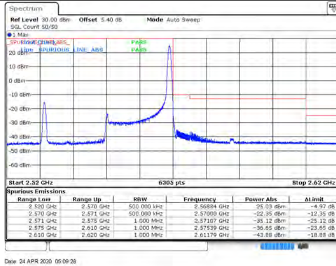
CA 7C 100RB+100RB 16QAM 21152+21350 100RB#0+100RB#0
