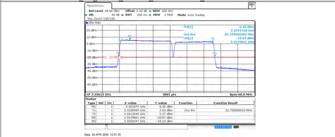
CA_7C_20+15_16QAM_21201+21372_100RB#0+75RB#0
