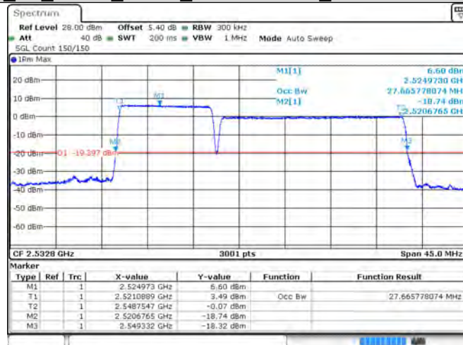
CA_7C_10+20_QPSK_21006+21150_50RB#0+100RB#0
