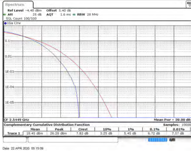
CA 7C 100RB+100RB 16QAM 21350+21152 100RB#0+100RB#0
