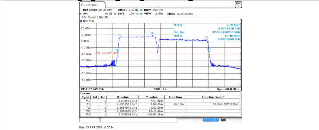
CA_7C_15+20_16QAM_20828+20999_75RB#0+100RB#0
