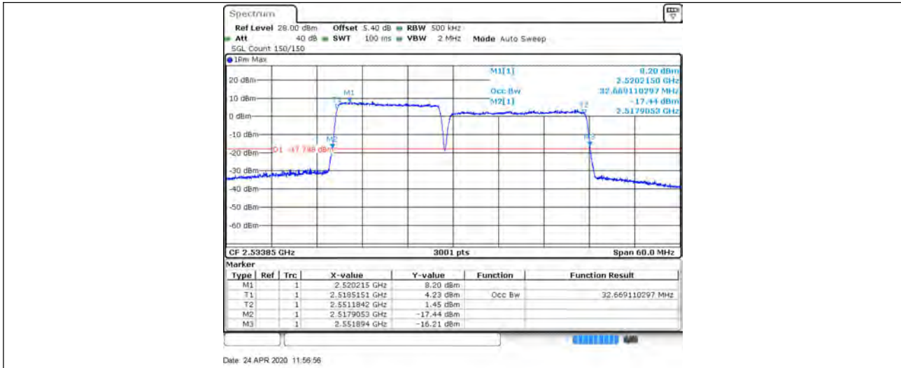
CA_7C_15+20_64QAM_21179+21350_75RB#0+100RB#0
