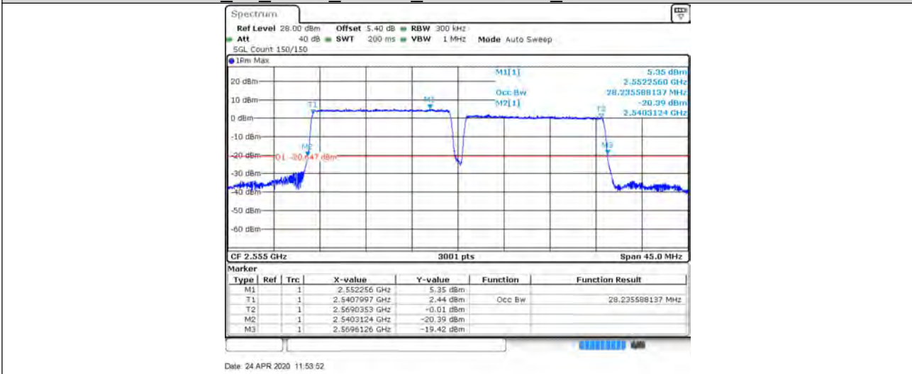
CA 7C_15+15_64QAM_20825+20975_75RB#0+75RB#0
