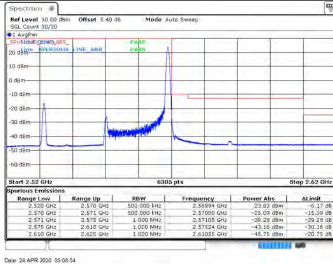
CA_7C_100RB+100RB_QPSK_21152+21350_100RB#0+100RB#0
