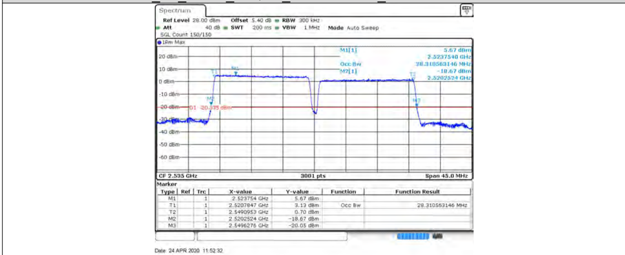
CA 7C_15+15_64QAM_21225+21375_75RB#0+75RB#0
