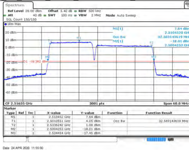
CA 7C_15+20_QPSK_21003+21174_75RB#0+100RB#0
