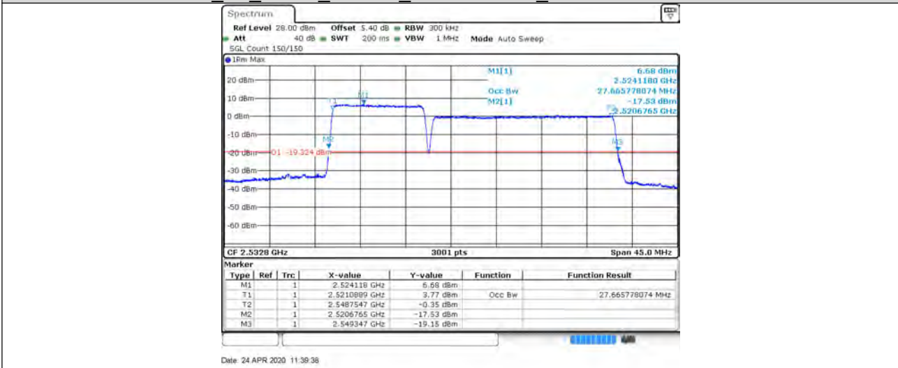
CA_7C_10+20_64QAM_21206+21350_50RB#0+100RB#0
