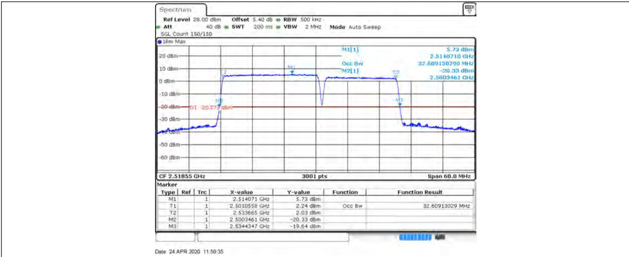
CA_7C_20+15_16QAM_21026+21197_100RB#0+75RB#0
