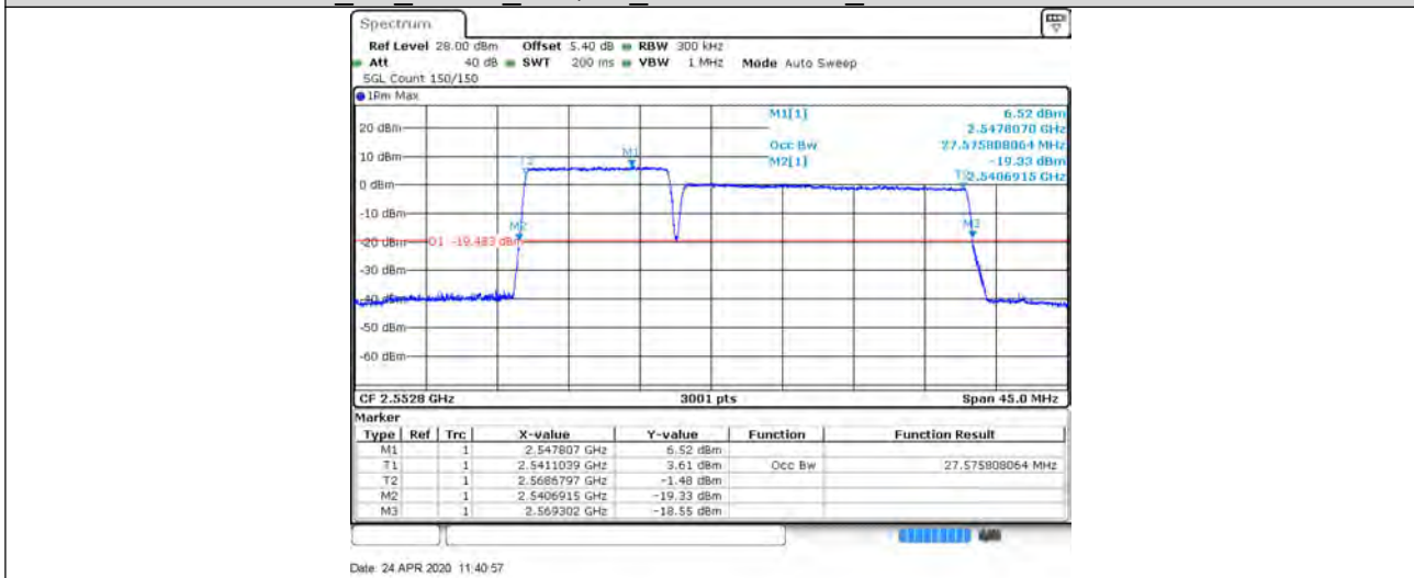
CA_7C_10+20_64QAM_20805+20949_50RB#0+100RB#0
