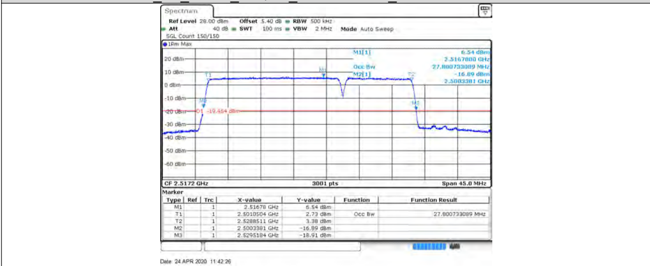
CA_7C_20+10_16QAM_21051+21195_100RB#0+50RB#0
