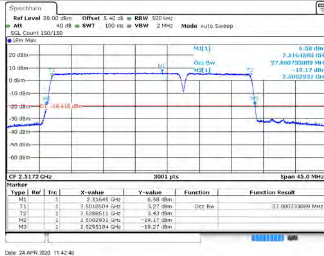
CA_7C_20+10_64QAM_21051+21195_100RB#0+50RB#0
