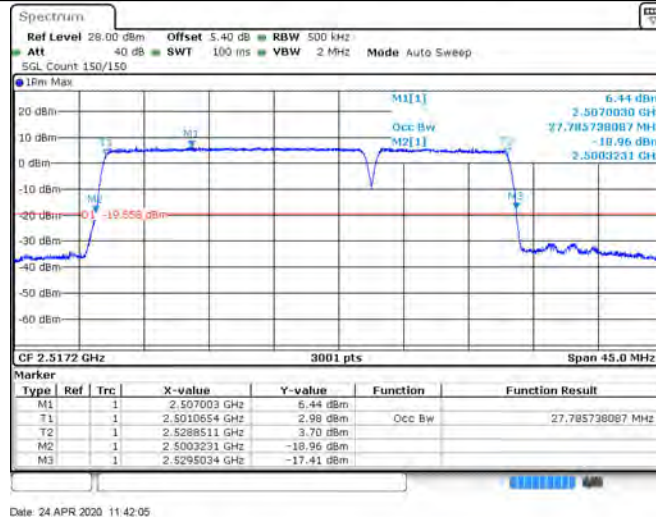
CA 7C_20+10_QPSK_21051+21195_100RB#0+50RB#0
