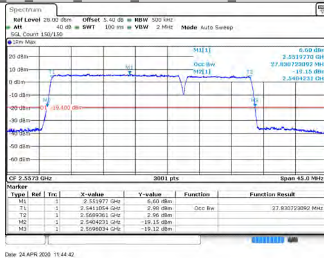
CA_7C_20+10_64QAM_20850+20994_100RB#0+50RB#0
