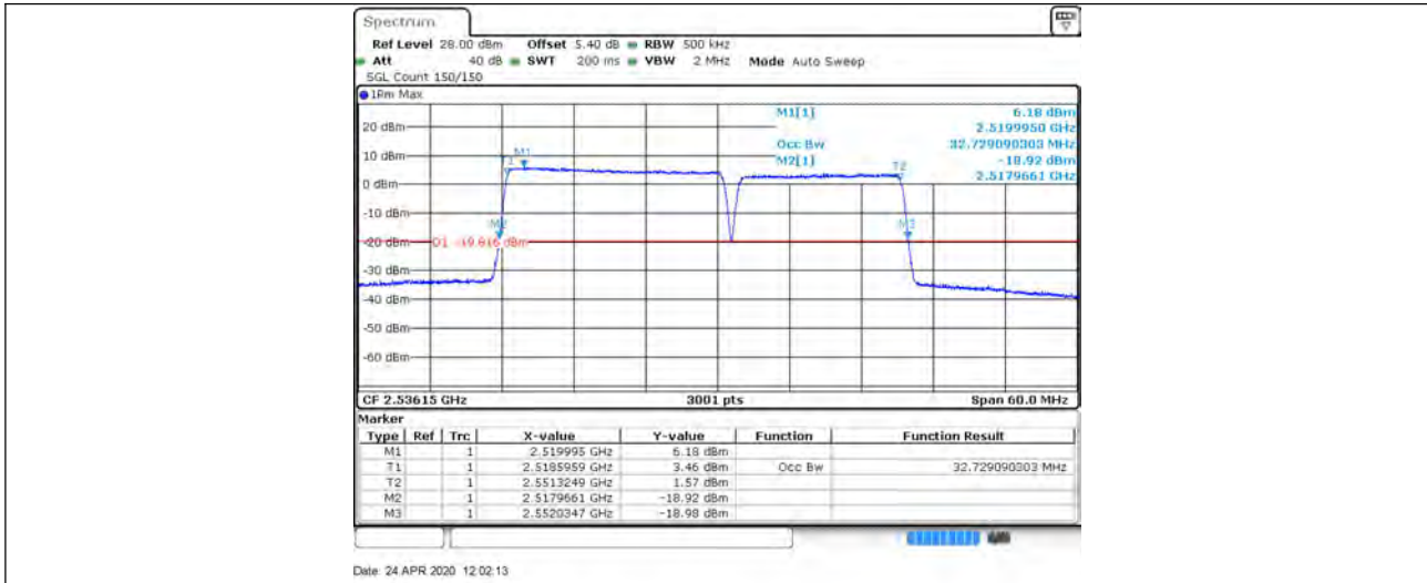
CA_7C_20+15_64QAM_21201+21372_100RB#0+75RB#0
