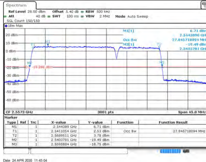
CA 7C_20+15_QPSK_20850+21021_100RB#0+75RB#0
