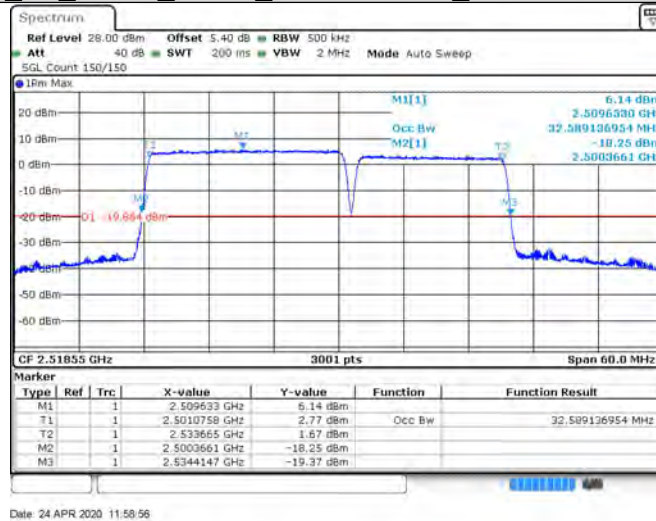
CA 7C_20+15_QPSK_21026+21197_100RB#0+75RB#0
