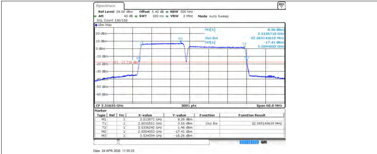
CA_7C_15+20_16QAM_21003+21174_75RB#0+100RB#0
