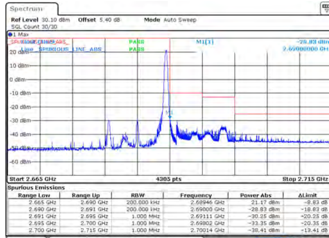
Band41_10MHz_16QAM_41540_50RB#0
