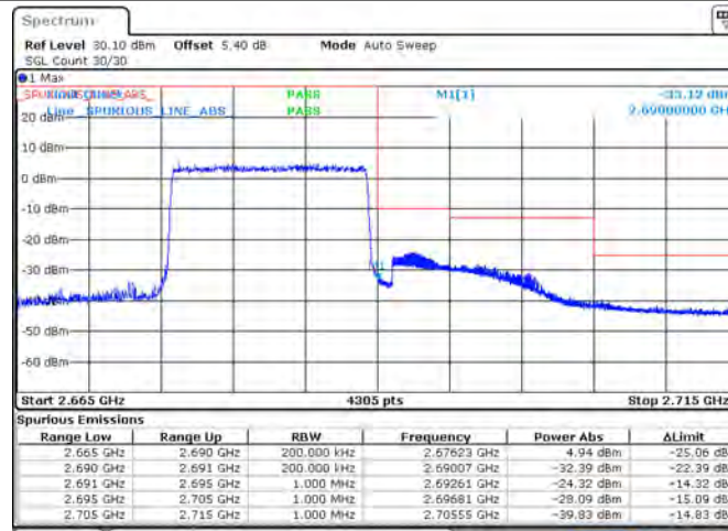
Band41_15MHz_16QAM_41515_75RB#0
