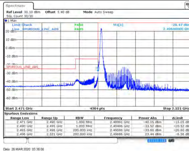
Band41_15MHz_16QAM_39725_75RB#0
