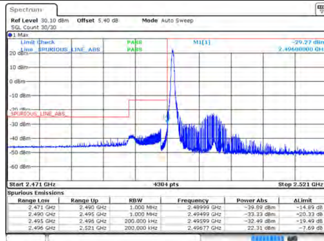
Band41_15MHz_64QAM_39725_75RB#0
