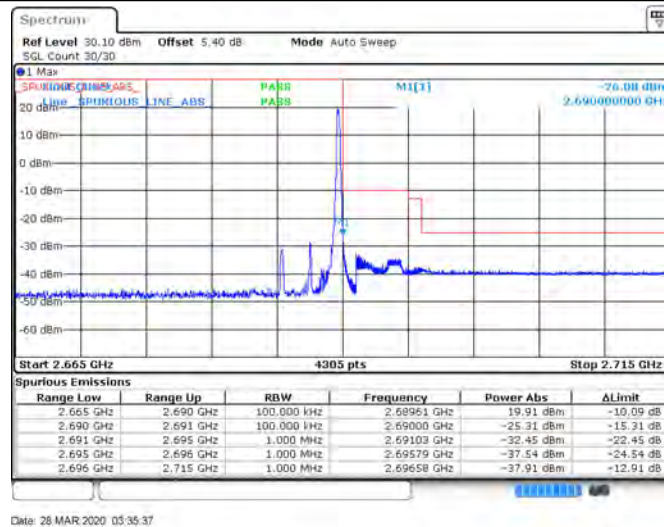
Band41_5MHz_64QAM_41565_25RB#0
