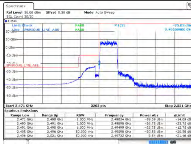
Band41_5MHz_QPSK_39675_25RB#0
